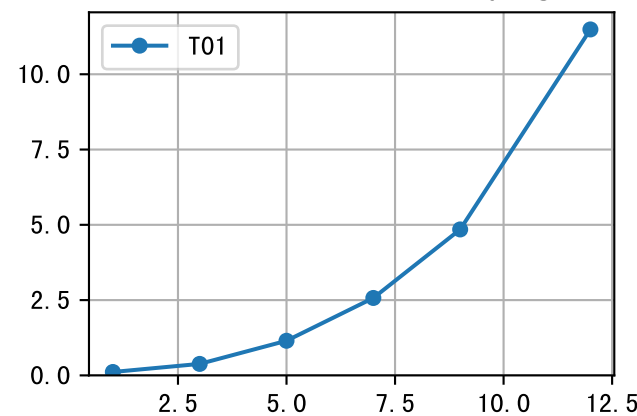
FrV (P3-021-19) Plot By Age
