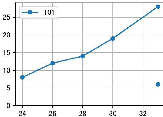
FrD (P3-068-4)
