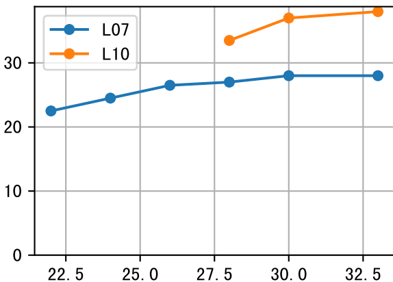
LfL (P3-068-4)
