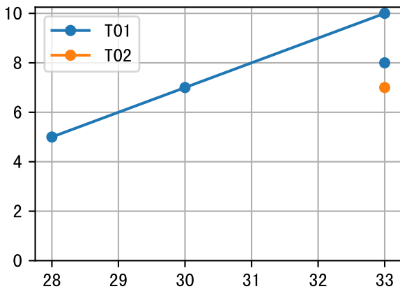
FrD (P3-075-19)
