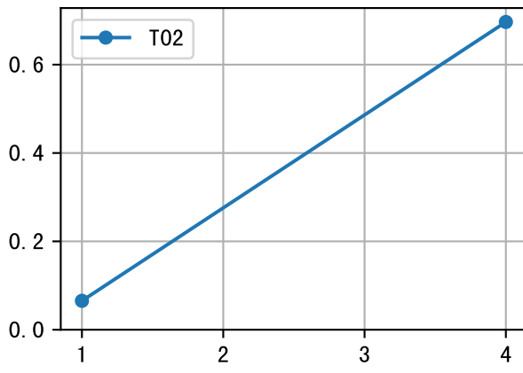
FrV (P3-034-5) Plot By Age
