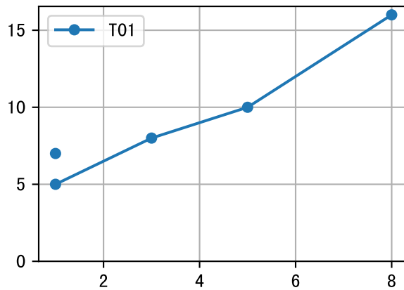
P3 (Raw data plots) FrD (P3-045-17) Plot By Age
