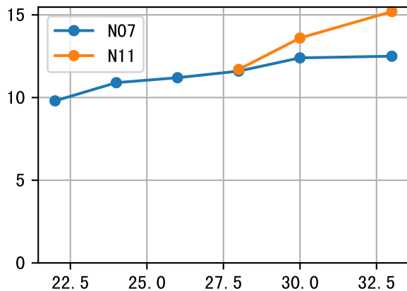
NdD (P3-075-19)
