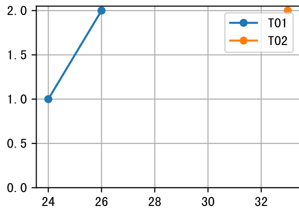
FrN (P3-054-28)
