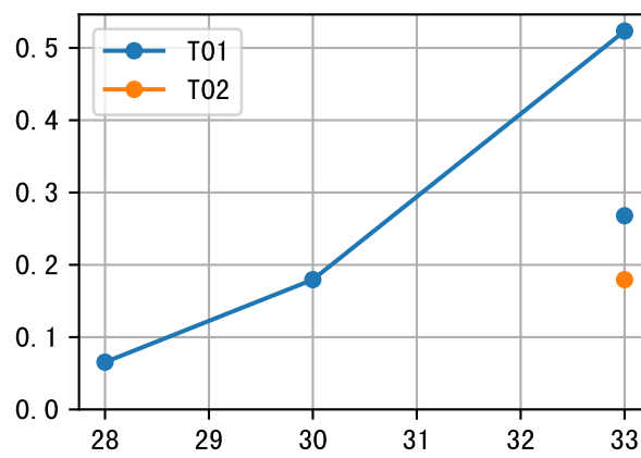
FrV (P3-075-19)
