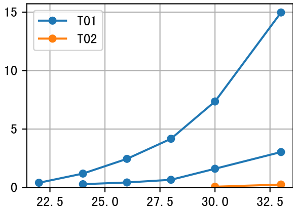
FrV (P3avg)
