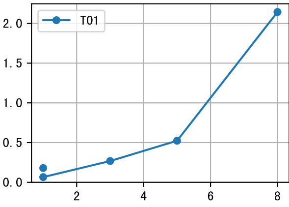
FrV (P3-045-17) Plot By Age
