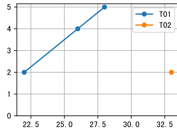
FrN (P3-110-23)
