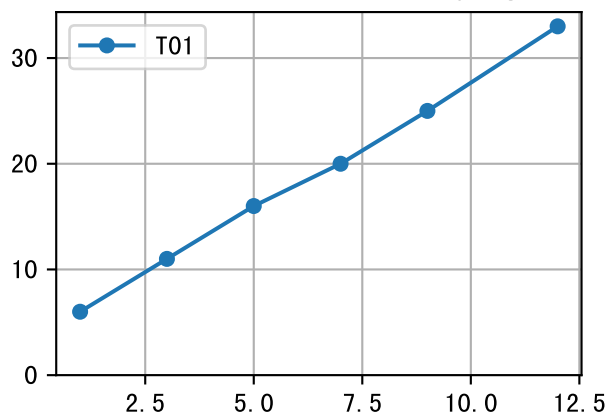
FrD (P3-084-11) Plot By Age
