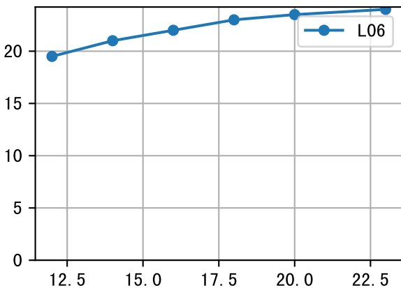
LfL (P3-045-17) Plot By Age
