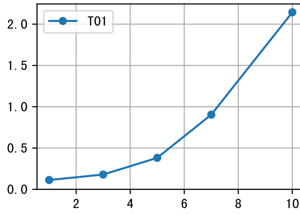
FrV (P3-054-28) Plot By Age
