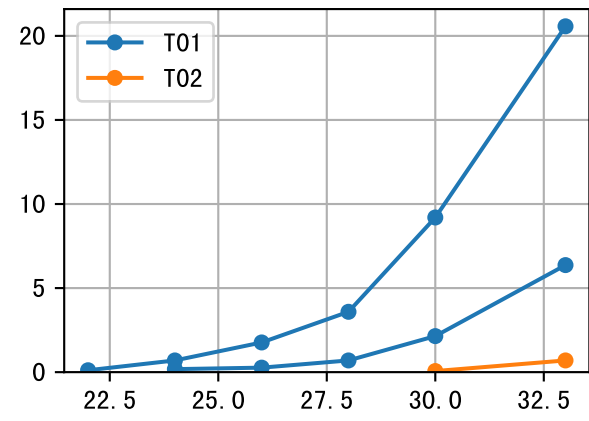
FrV (P3-034-5)
