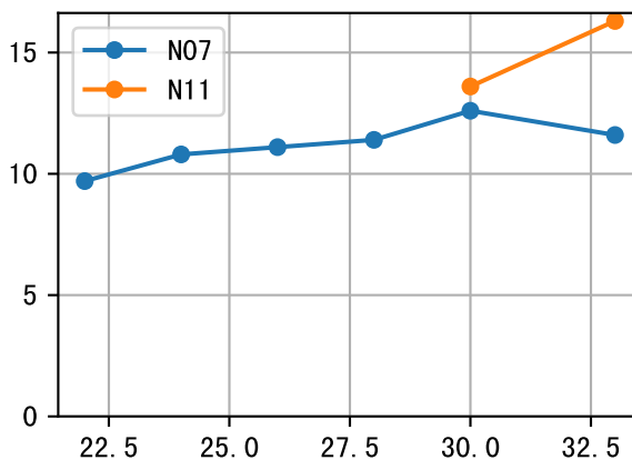
NdD (P3-099-4)
