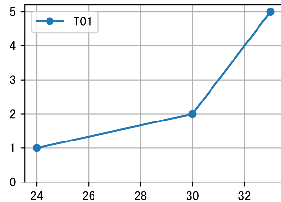
FrN (P3-068-4)
