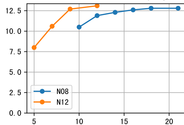
NdD (P3-054-28) Plot By Age
