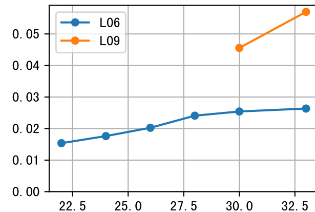
LfA (P3-099-4)
