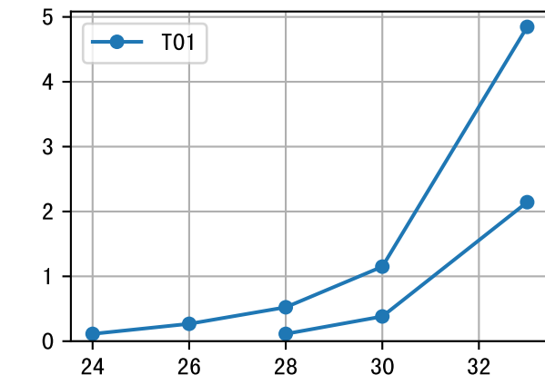
FrV (P3-099-4)
