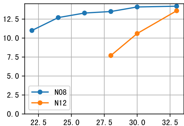
NdD (P3-068-4)
