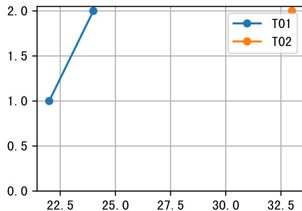
FrNR (P3-021-19)
