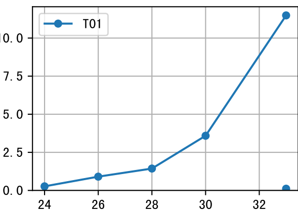
FrV (P3-068-4)
