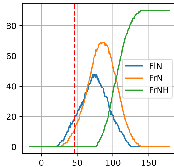
P5: ['FIN', 'FrN', 'FrNH']
