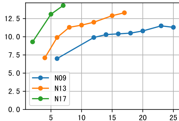
NdD (P6AE-014-17) Plot By Age
