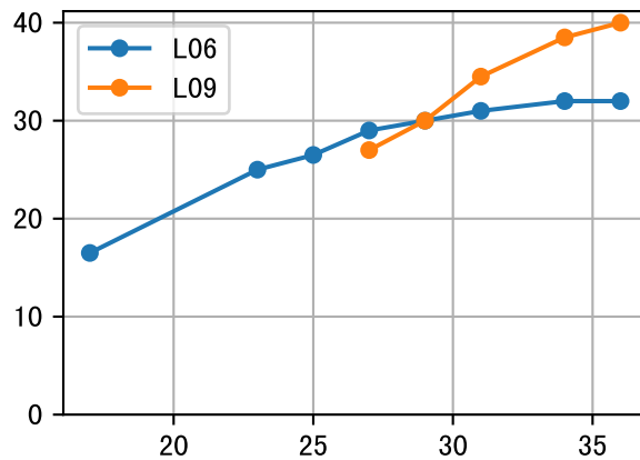
P6AE (Raw data plots) LFW (P6AE-007-16)
