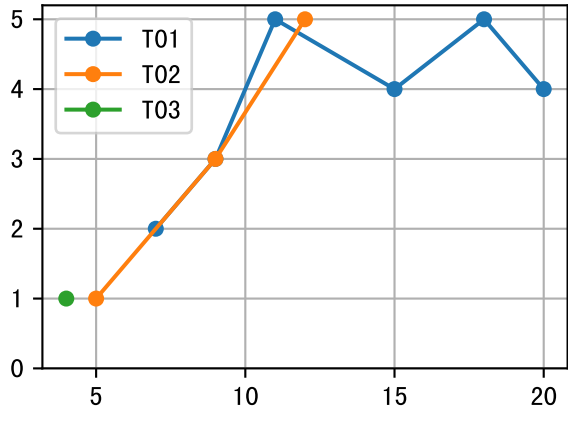
FrNR (P6AE-014-17) Plot By Age
