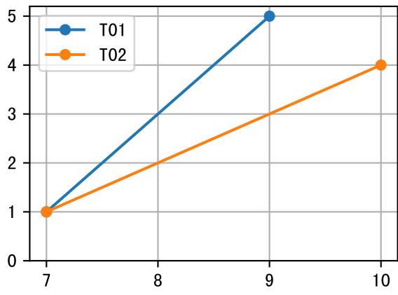
FrN (P6AE-033-4) Plot By Age
