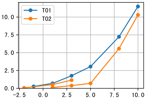
FrV (P6AE-014-17) Plot By Age
