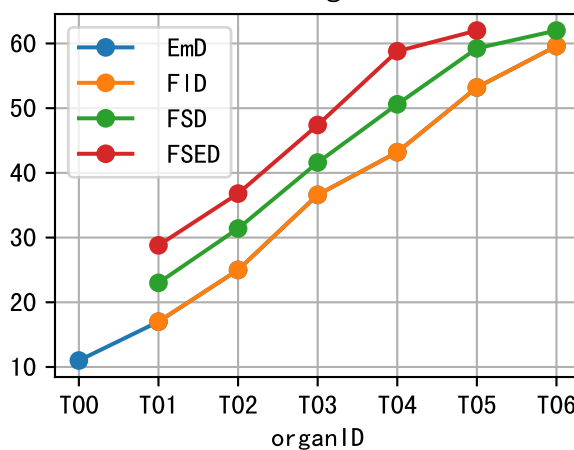
P6AEavg Phe
