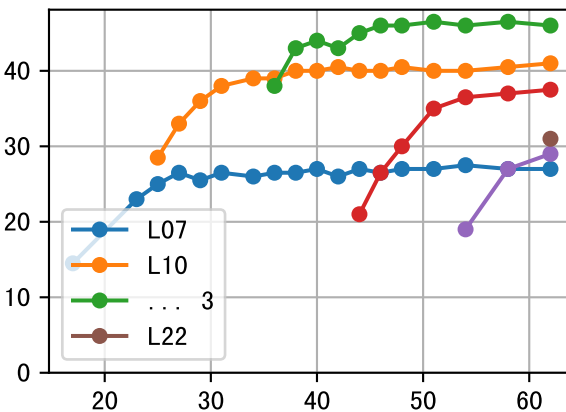
LfL (P6AE-026-25)
