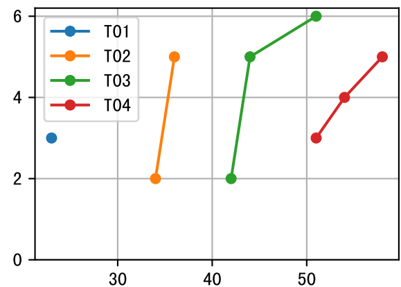
FrN (P6AE-007-10)
