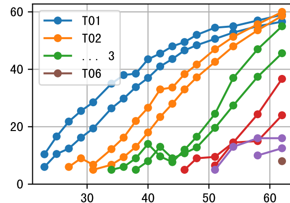
FrD (P6AEavg)
