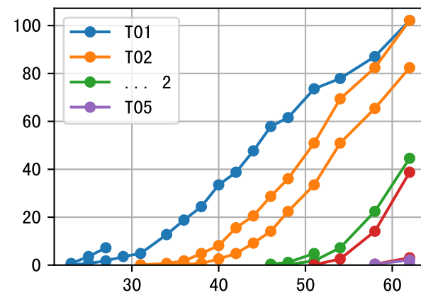
FrV (P6AE-045-12)
