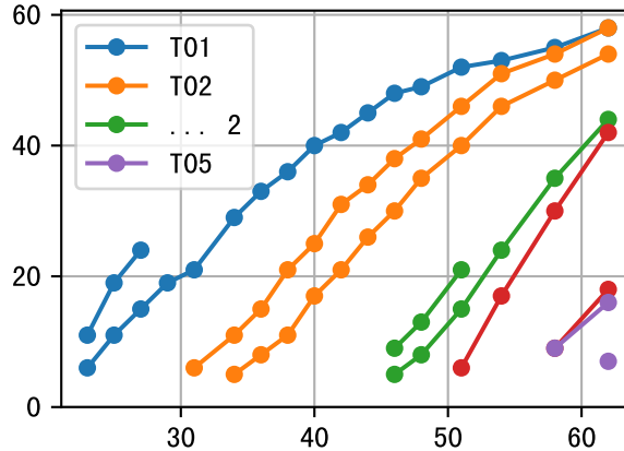
FrD (P6AE-045-12)
