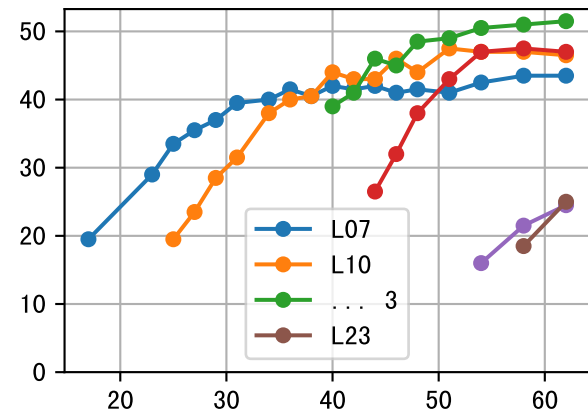
LFW (P6AE-045-12)
