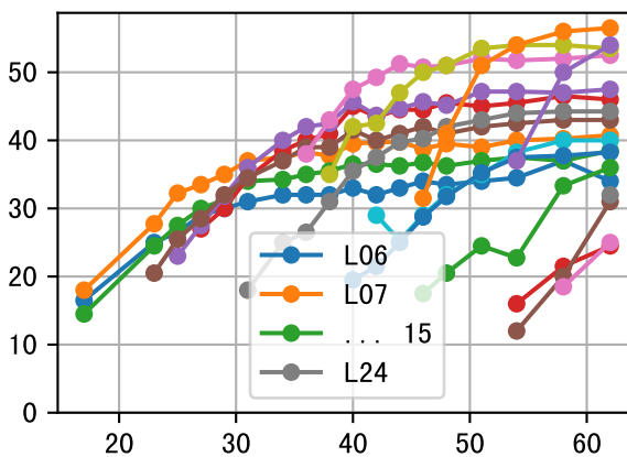
LfW (P6AEavg)
