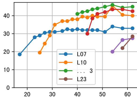
LfL (P6AE-045-12)
