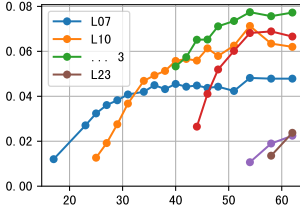
LfA (P6AE-045-12)
