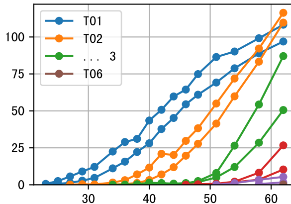
FrV (P6AEavg)
