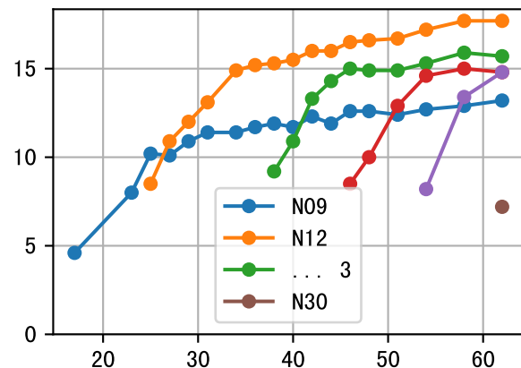
NdD (P6AE-033-4)
