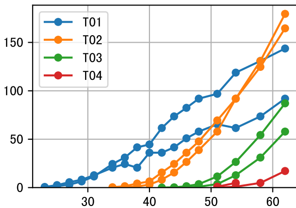
FrV (P6AE-007-10)
