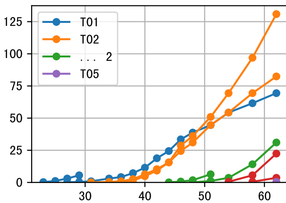
FrV (P6AE-033-4)
