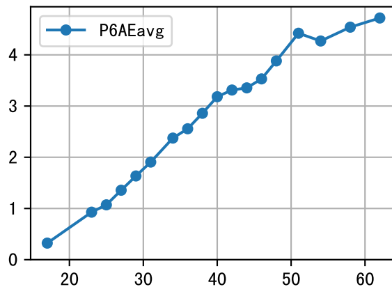
LAI
