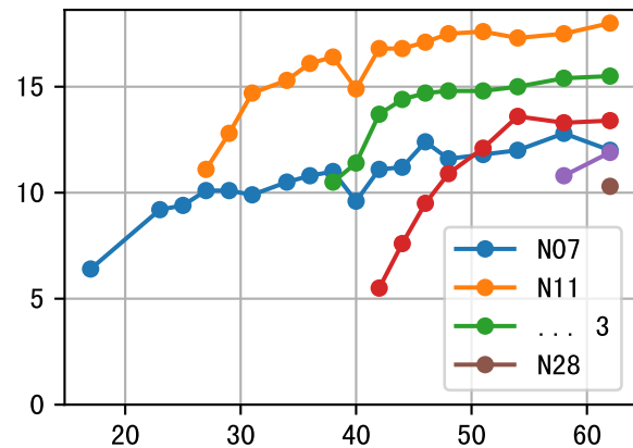
NdD (P6AE-007-10)
