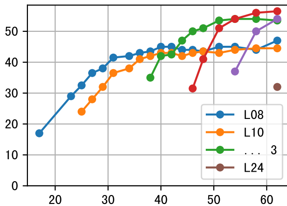
LfW (P6AE-033-4)
