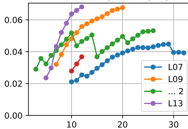
P6AW (Avg data plots) LIA (P6AWavg) Plot By Age
