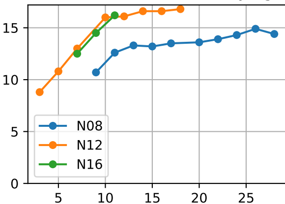
NdD (P6AW-095-29) Plot By Age
