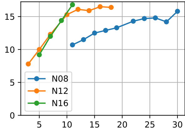
NdD (P6AW-074-9) Plot By Age
