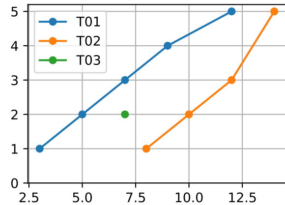
FrN (P6AW-074-9) Plot By Age
