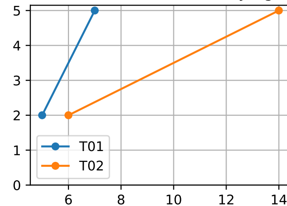
FrN (P6AW-058-22) Plot By Age
