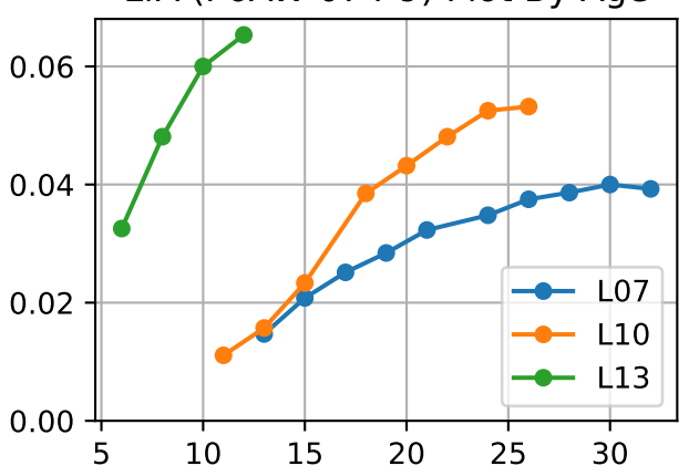
LfA (P6AW-074-9) Plot By Age
