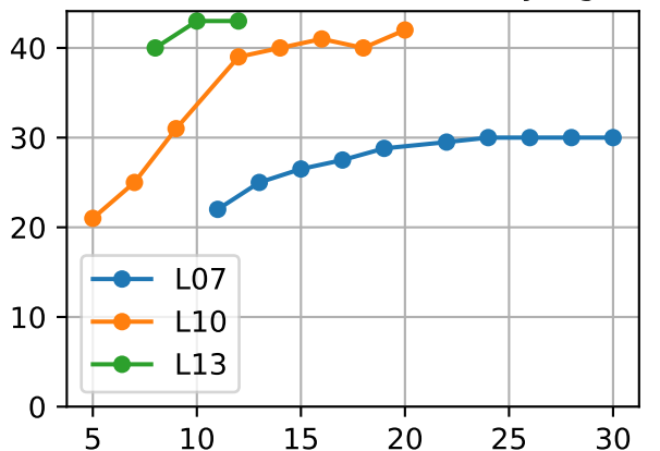
LfL (P6AW-095-29) Plot By Age
