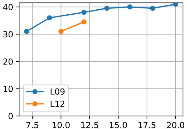
LfL (P6AW-058-22) Plot By Age
