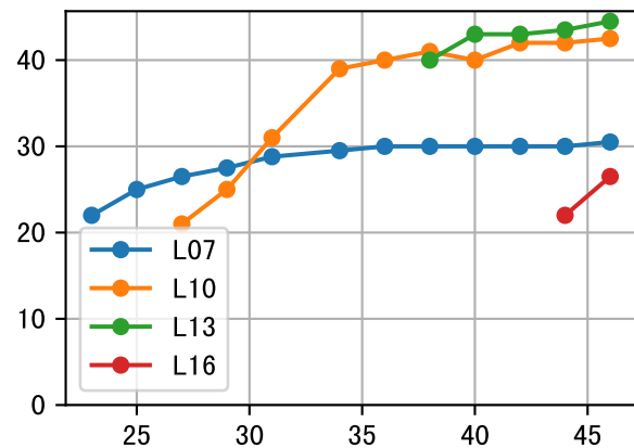
LfL (P6AW-095-29)
