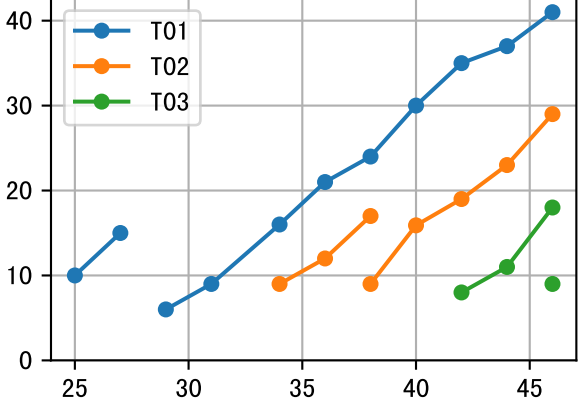
FrD (P6AW-074-9)
