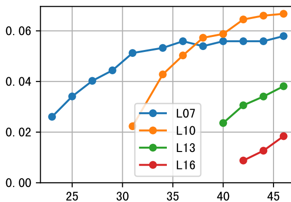
LfA (P6AW-106-11)
