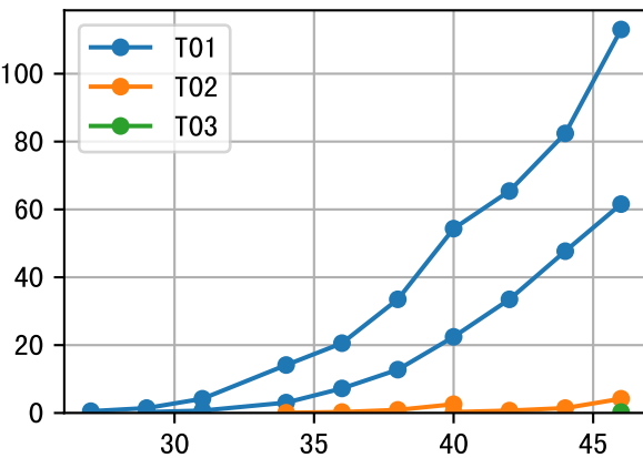
FrV (P6AW-058-22)
