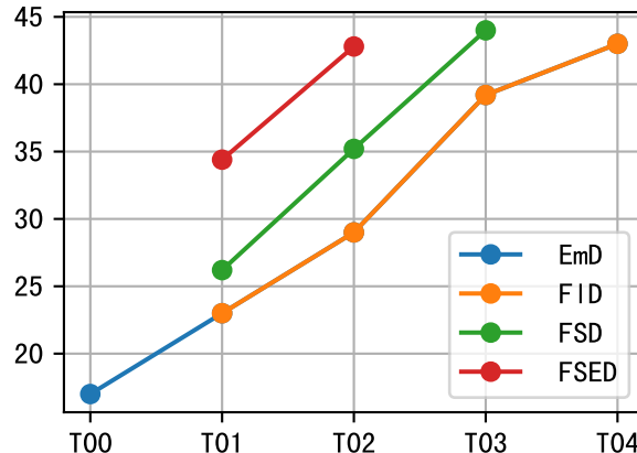
P6AWavg Phe
