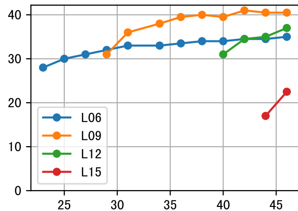
LfL (P6AW-058-22)
