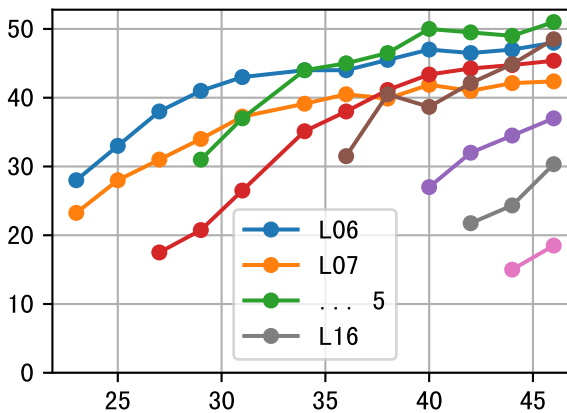
LfW (P6AWavg)
