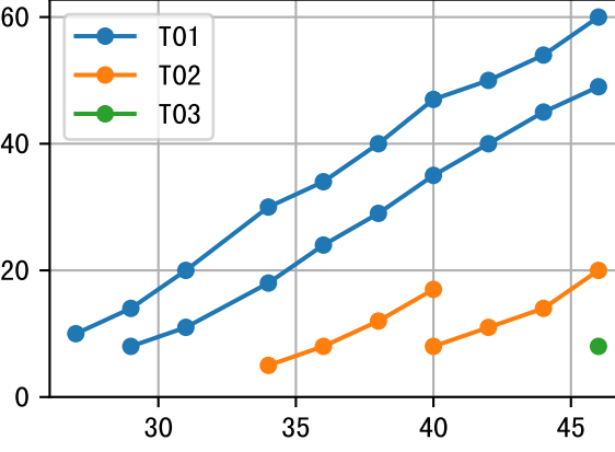
FrD (P6AW-058-22)
