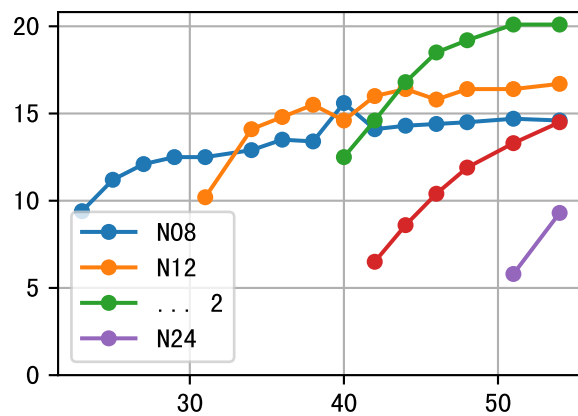
P6AW (Raw data plots) NdD (P6AW-106-11)
