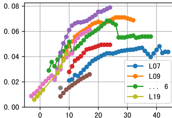
P6AW (Avg data plots) LfA (P6AWavg) Plot By Age
