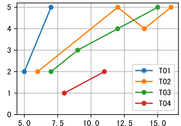
FrNR (P6AW-058-22) Plot By Age
