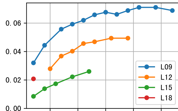
LfA (P6AW-058-22) Plot By Age
