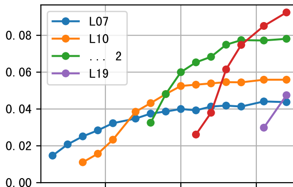
P6AW (Raw data plots)
