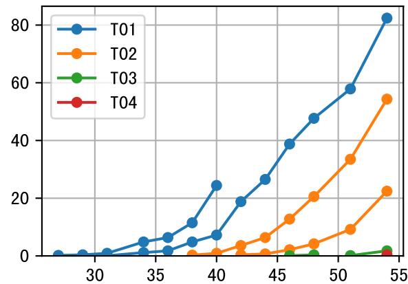
P6AW (Raw data plots) FrV (P6AW-087-14)
