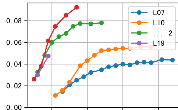
LfA (P6AW-074-9) Plot By Age
