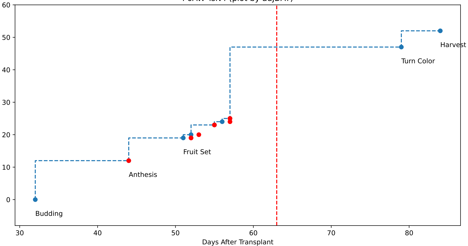
P6AW TsN4 (plot by adjDAT)
