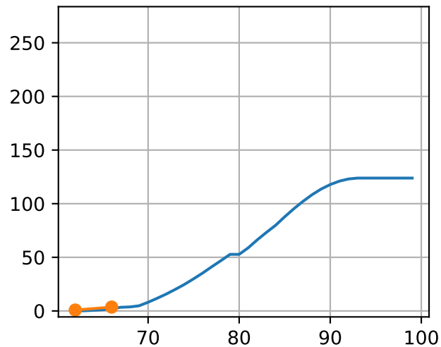
['S1T5Fr5']
