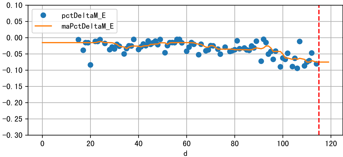
Daily %DeltaM and %DeltaM/1000ml ETcIdef for M_E (-7.5%/D, -9.3%/1000ml ET)
