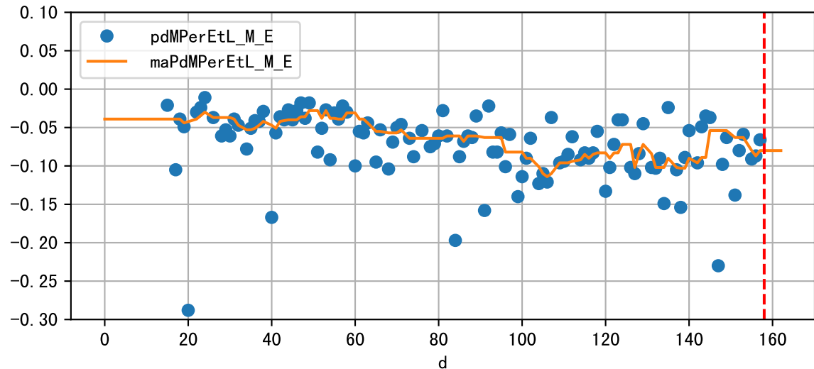
Daily %DeltaM and %DeltaM/1000ml ETcIdef for M_E (-9.1%/D, -8.0%/1000ml ET)
