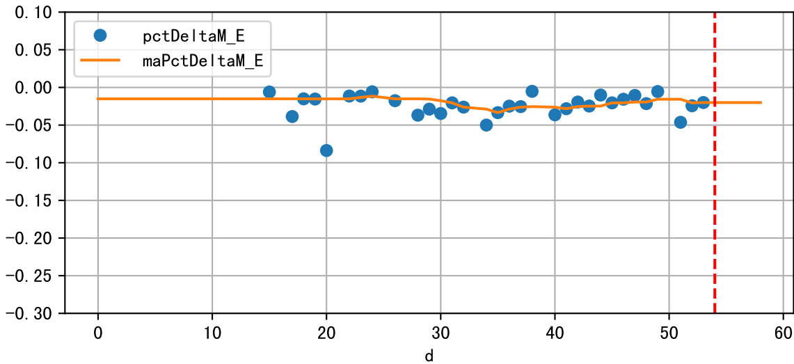
Daily %DeltaM and %DeltaM/1000ml ETcIdef for M_E (-2.0%/D, -3.6%/1000ml ET)
