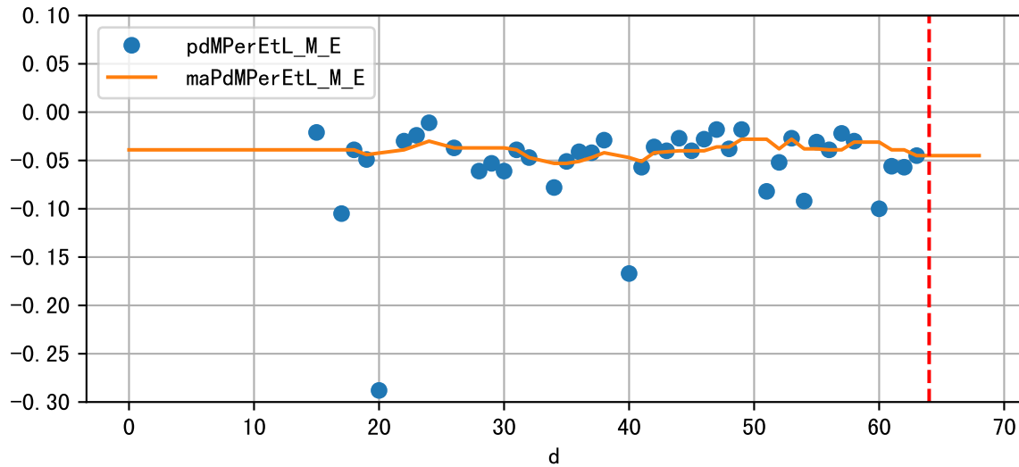
Daily %DeltaM and %DeltaM/1000ml ETcIdef for M_E (-1.6%/D, -4.5%/1000ml ET)
