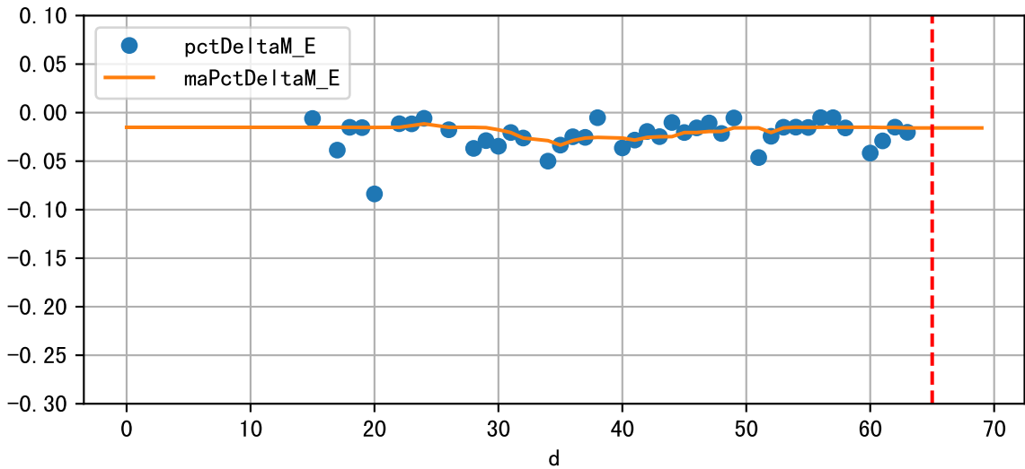
Daily %DeltaM and %DeltaM/1000ml ETcIdef for M_E (-1.6%/D, -4.4%/1000ml ET)
