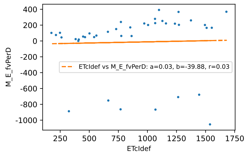
M_E daily ETcldef vs estFv (avgPctDeltaM = -4.3%)
