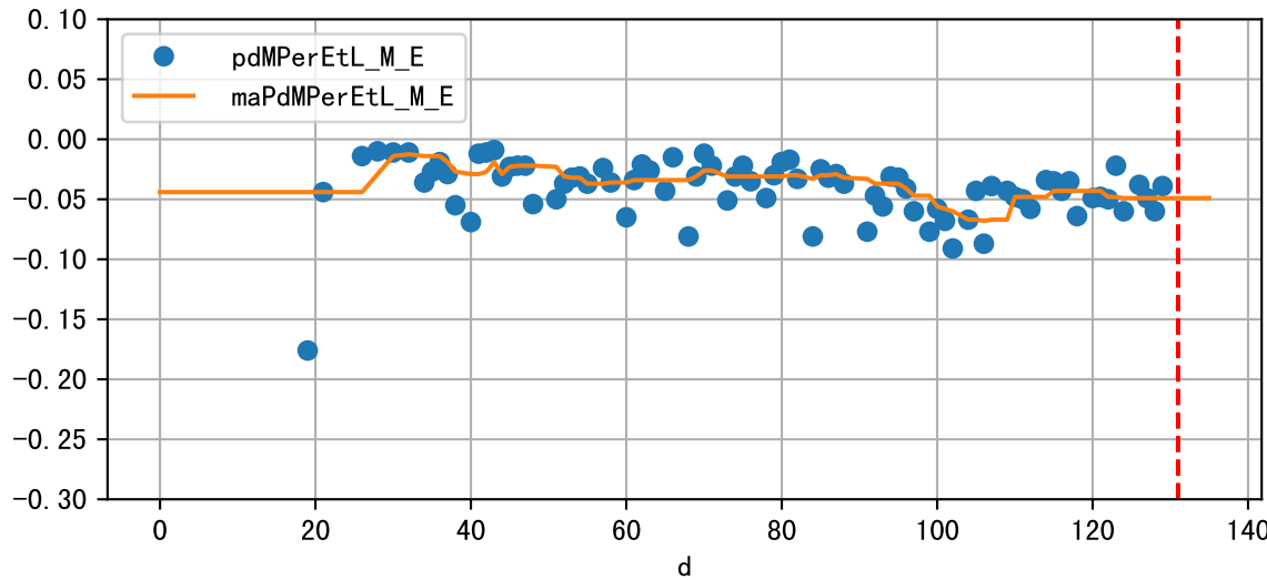
Daily %DeltaM and %DeltaM/1000ml ETcIdef for M_E (-4.1%/D, -4.9%/1000ml ET)
