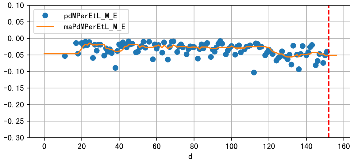
Daily %DeltaM and %DeltaM/1000ml ETcIdef for M_E (-4.9%/D, -5.1%/1000ml ET)
