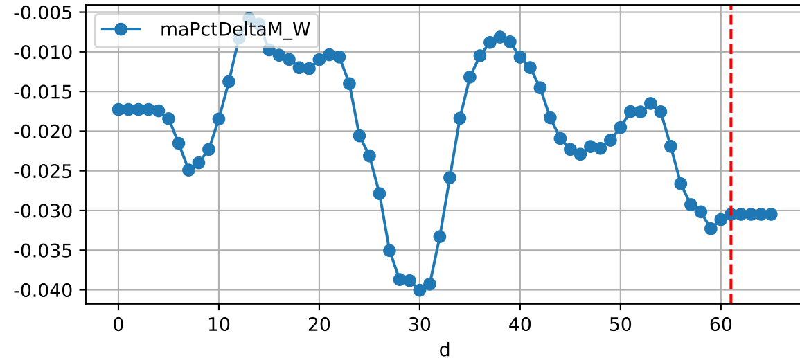
Daily %DeltaM and %DeltaM/1000ml ETcIdef for M_W (-3.0%/D, -2.5%/1000ml ET)
