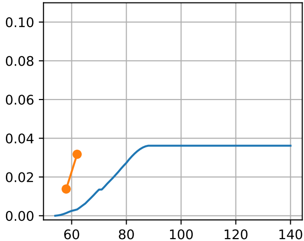
['S1L20']
