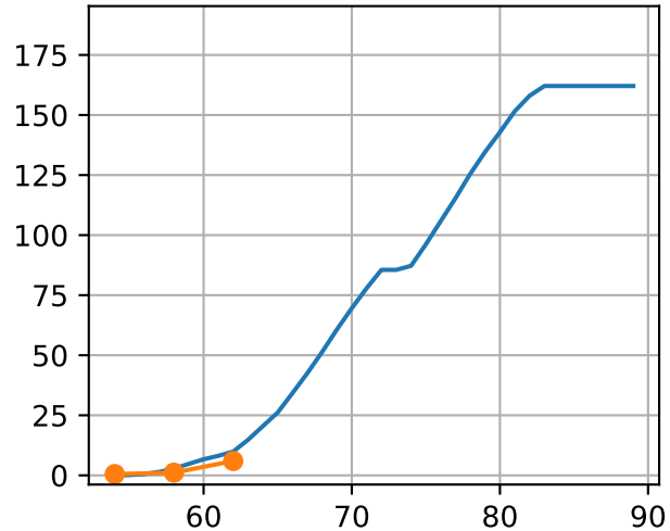
['S1T4Fr1']
