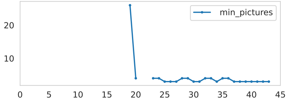
day_single
