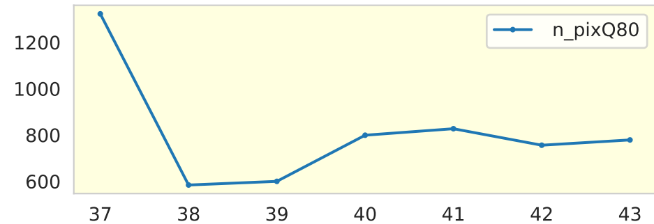
n_pixQ80 day
