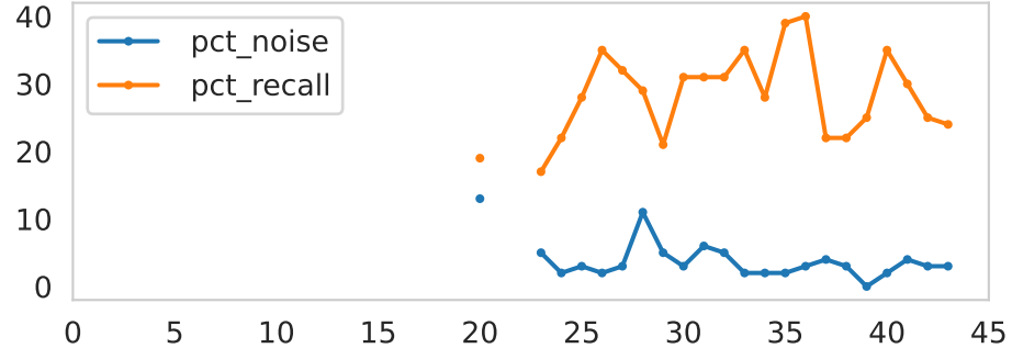
day_single
