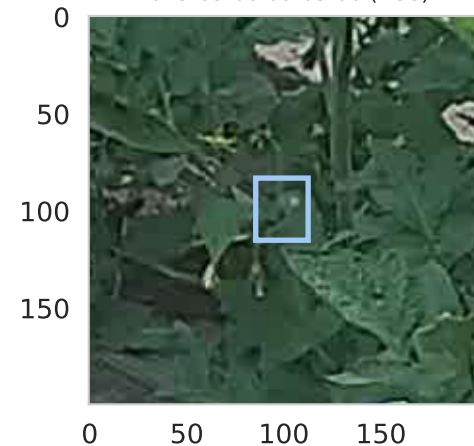
2025-05-10 11:55:00 (D40)
