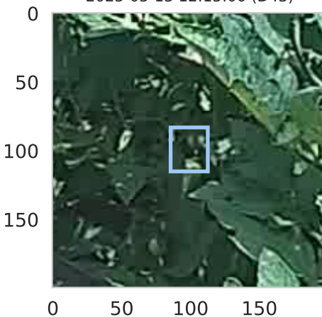
2025-05-13 12:15:00 (D43)
