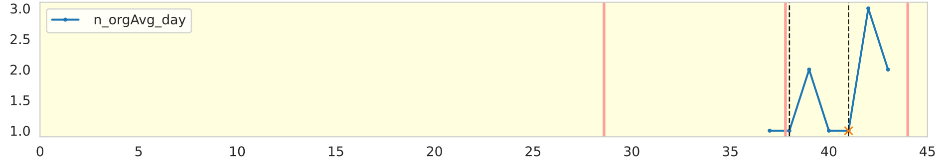
n_orgAvg day
