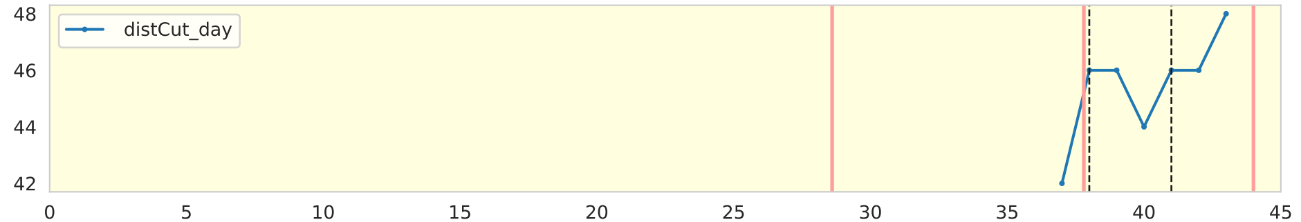
distCut day
