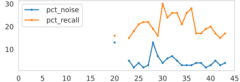
day_ward
