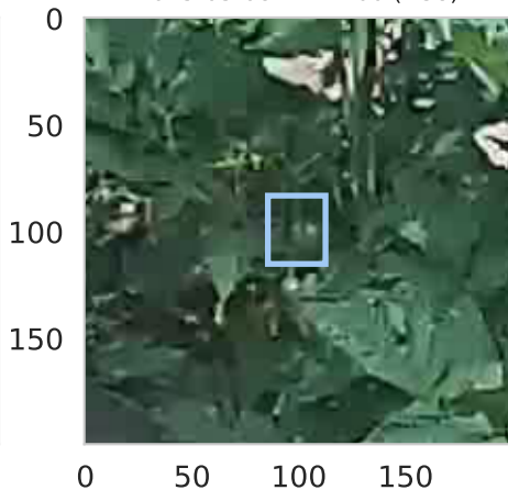
2025-05-13 09:04:00 (D43)
