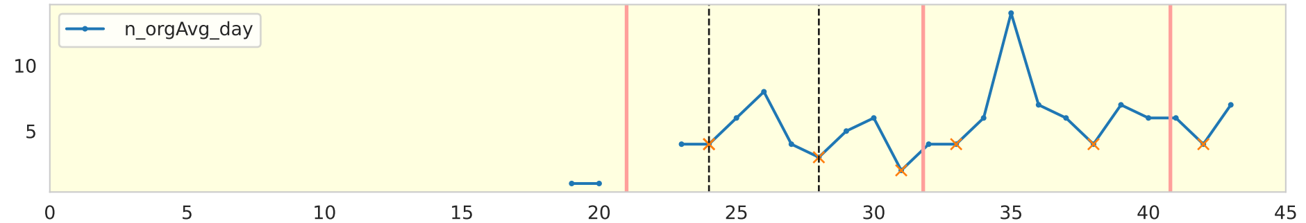
n_orgAvg day
