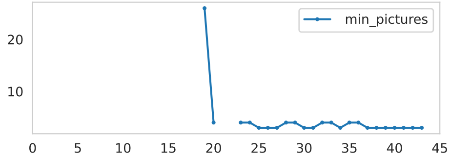
day_ward
