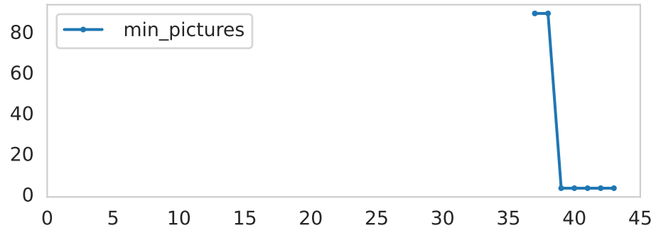
day_single
