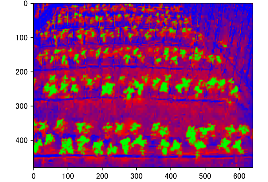
TGI
