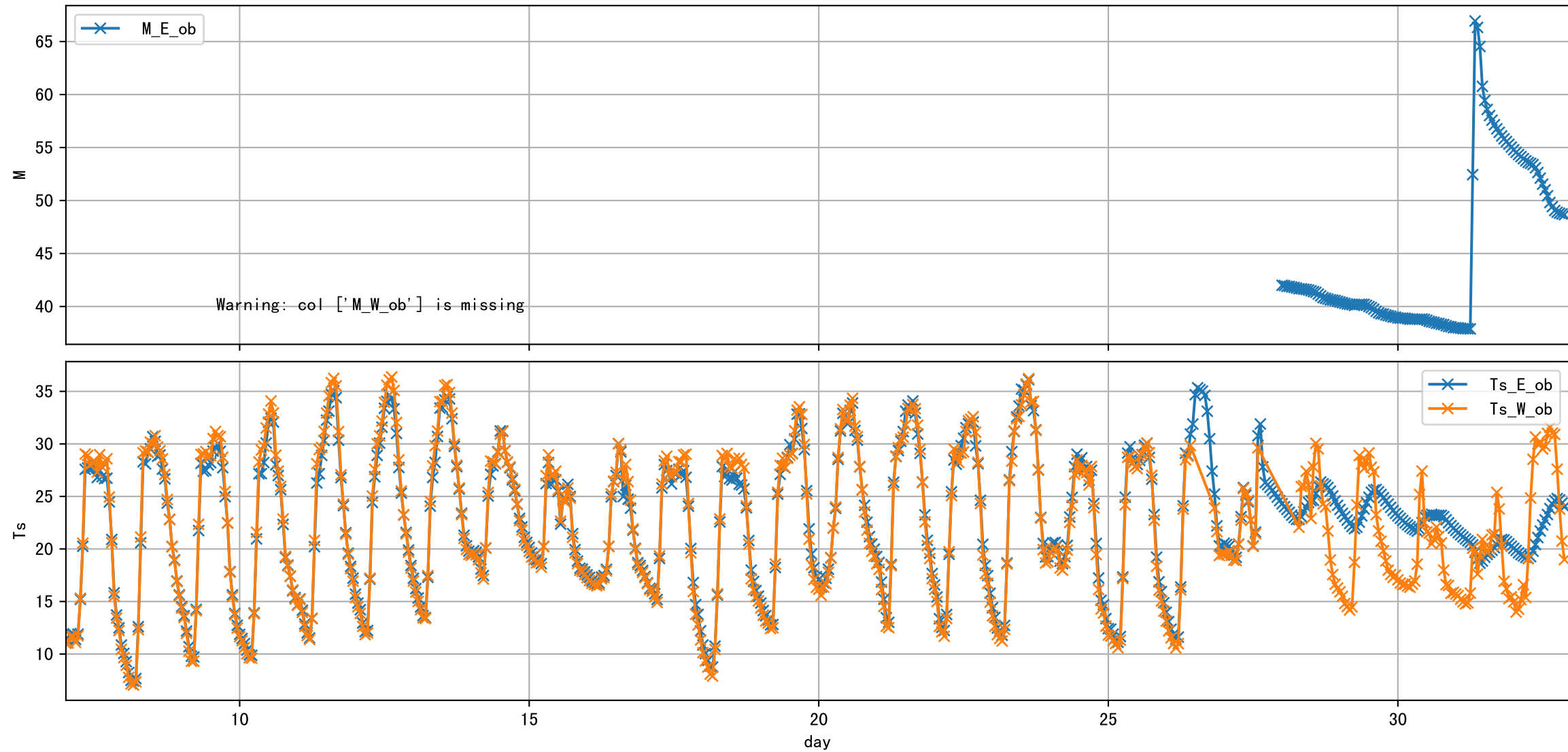
G1 2025-05-16 IS Observed Sensor Data
