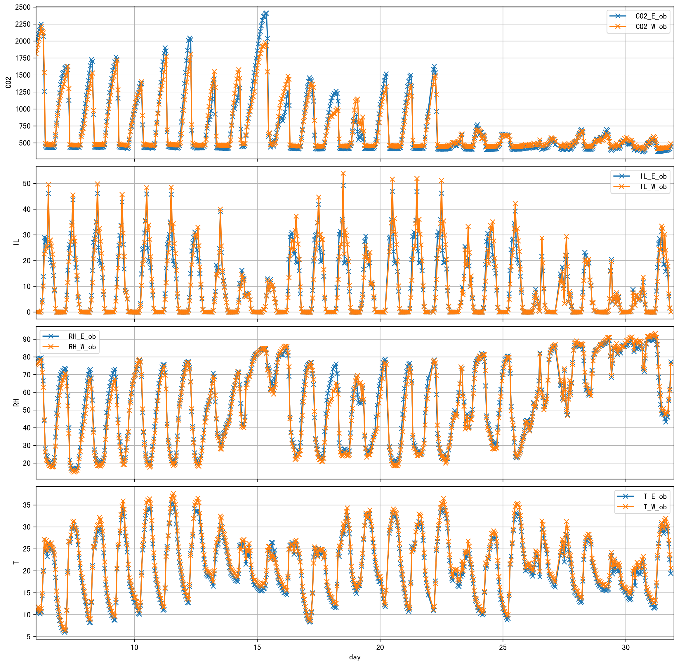
G3-13 2025-05-17 IA Observed Sensor Data
