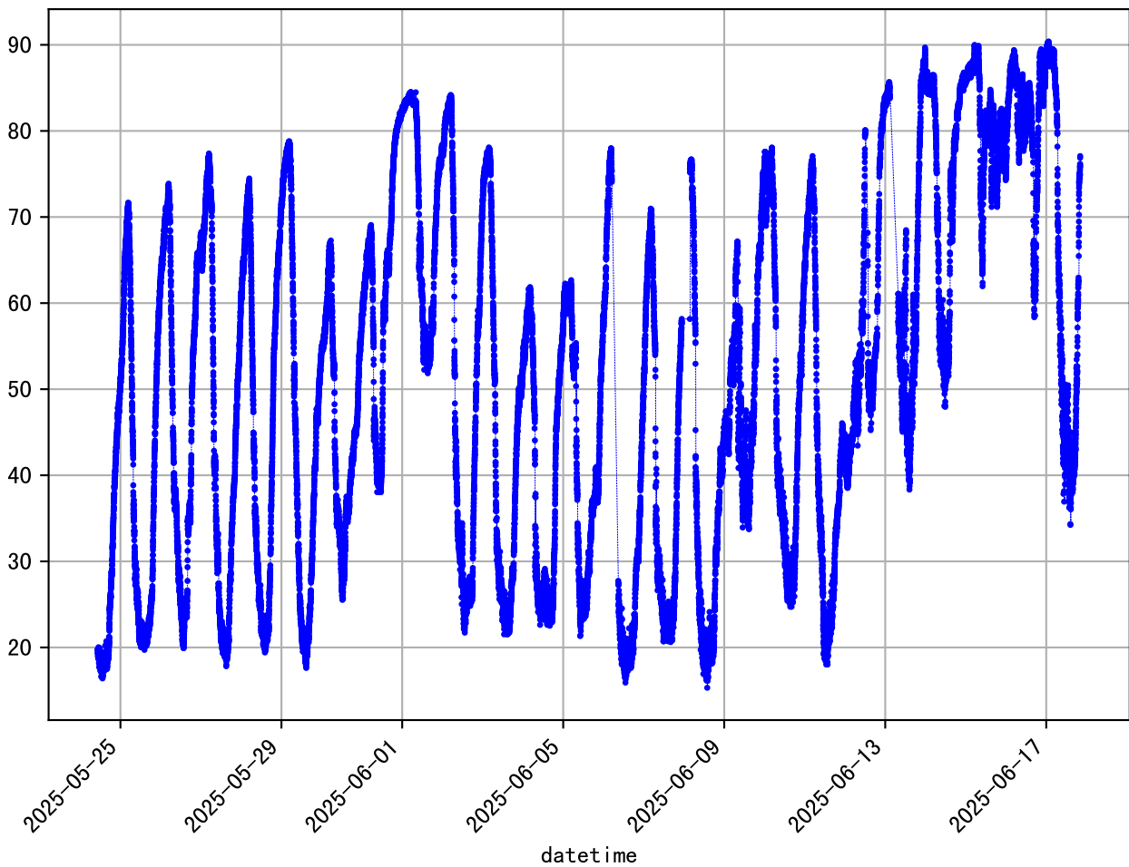
'Raw' data (24 days, 1 min/dp) 104115@1040661A_RH_E
