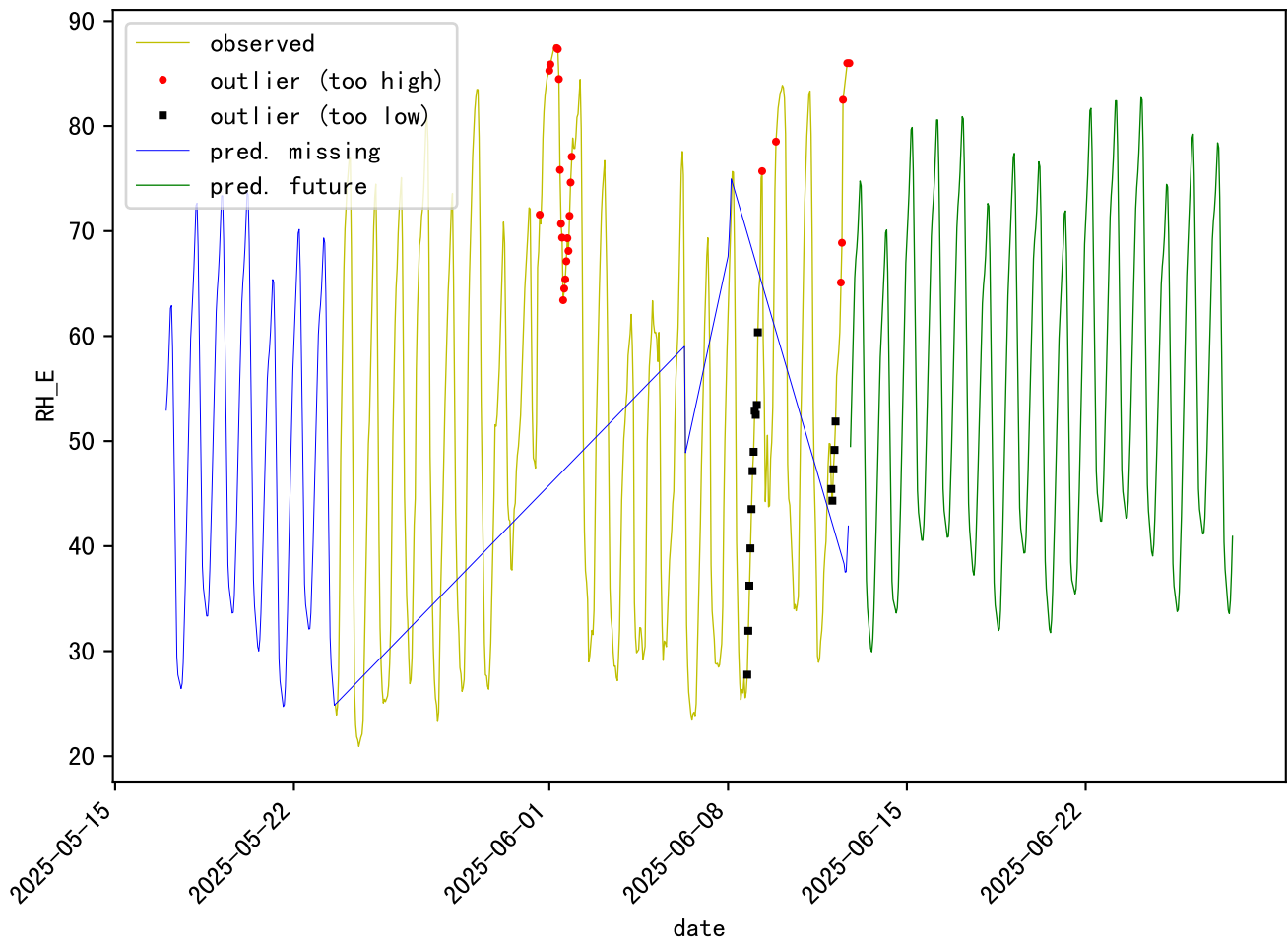
Model Prediction (H plot)
