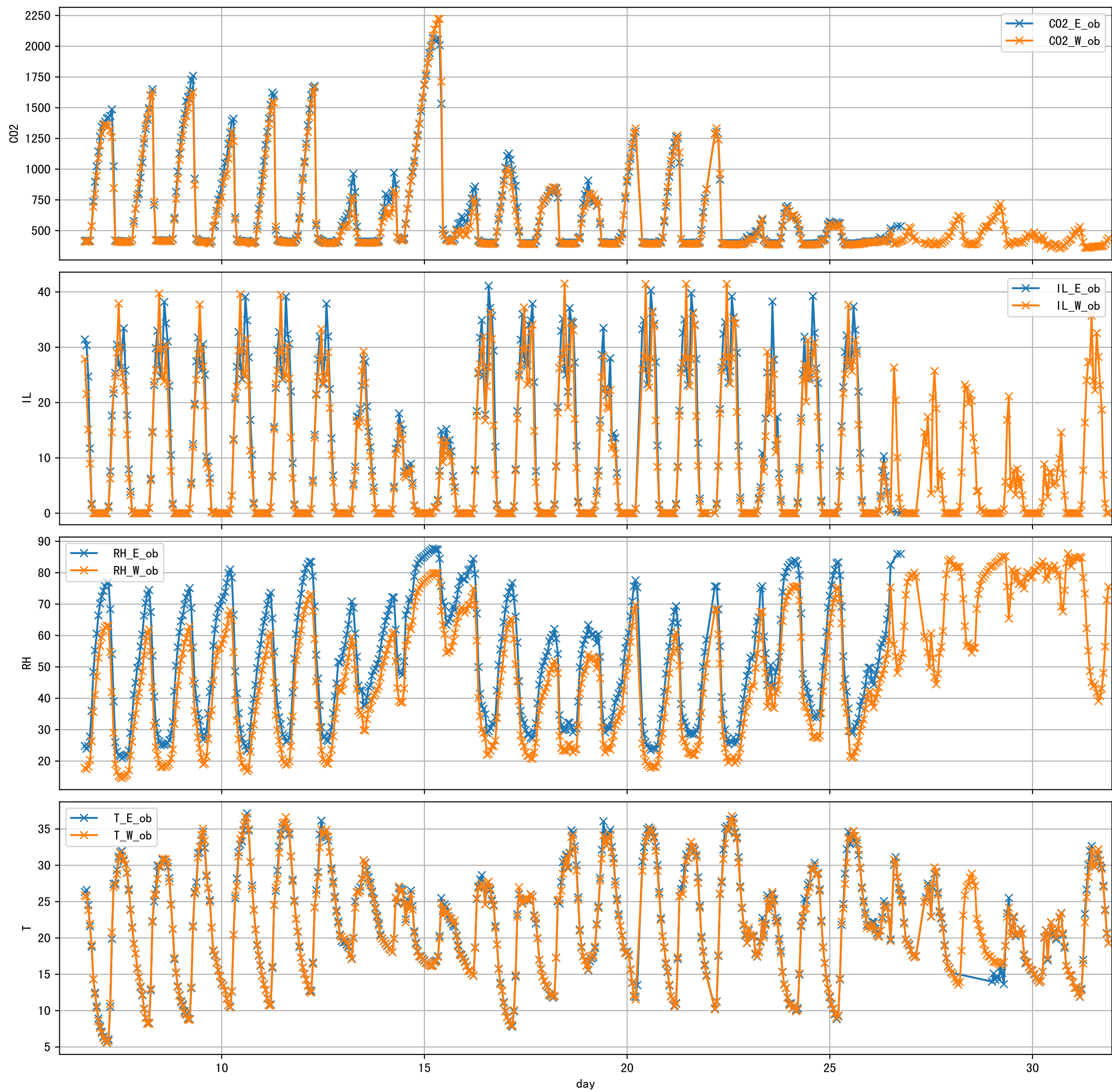
G3-16 2025-05-17 IA Observed Sensor Data
