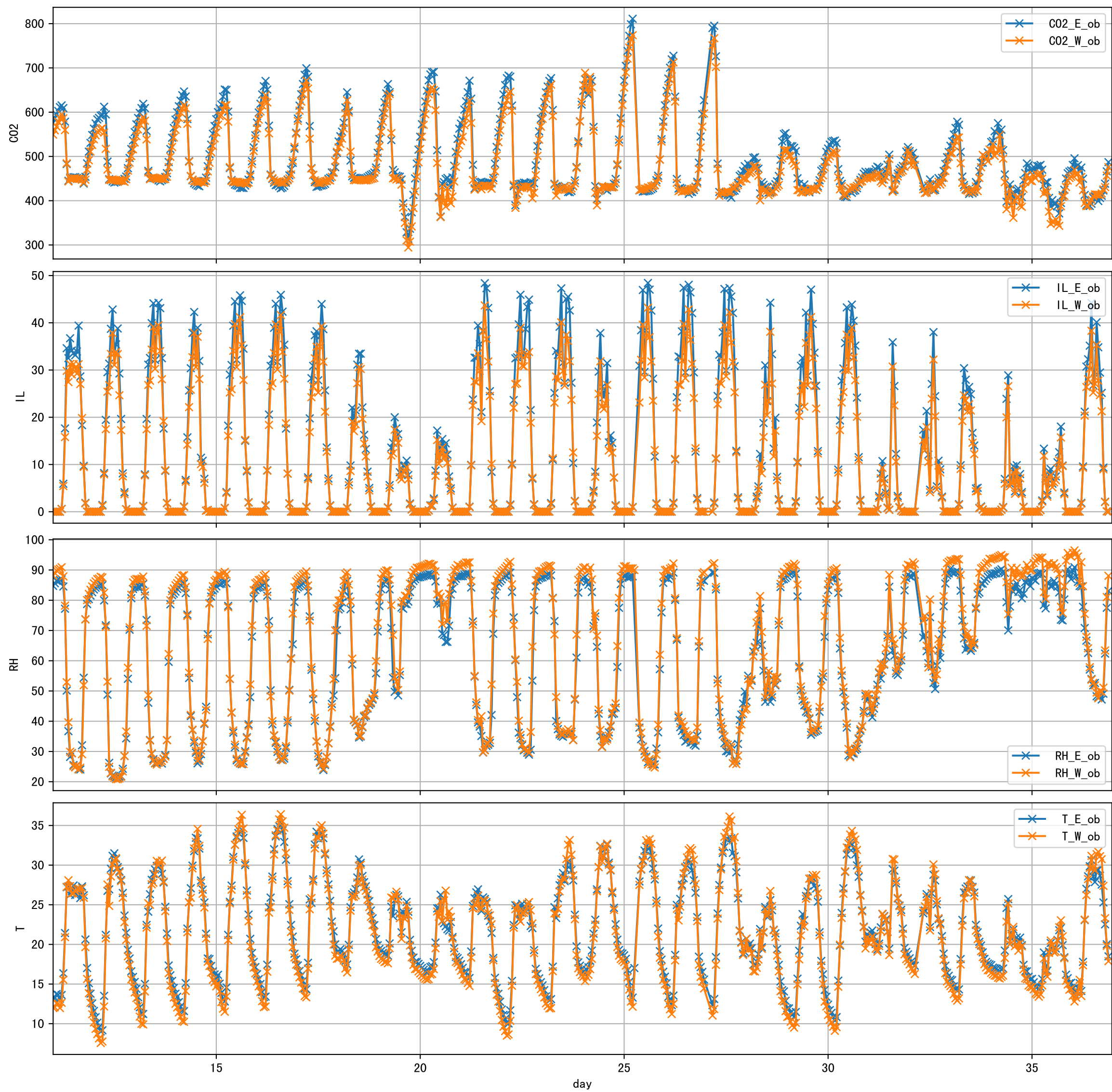
G3-1 2025-05-12 IA Observed Sensor Data
