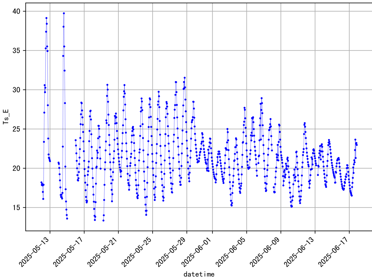
'H' data (36 days, 64 min/dp) 101533@101484IS_Ts_E
