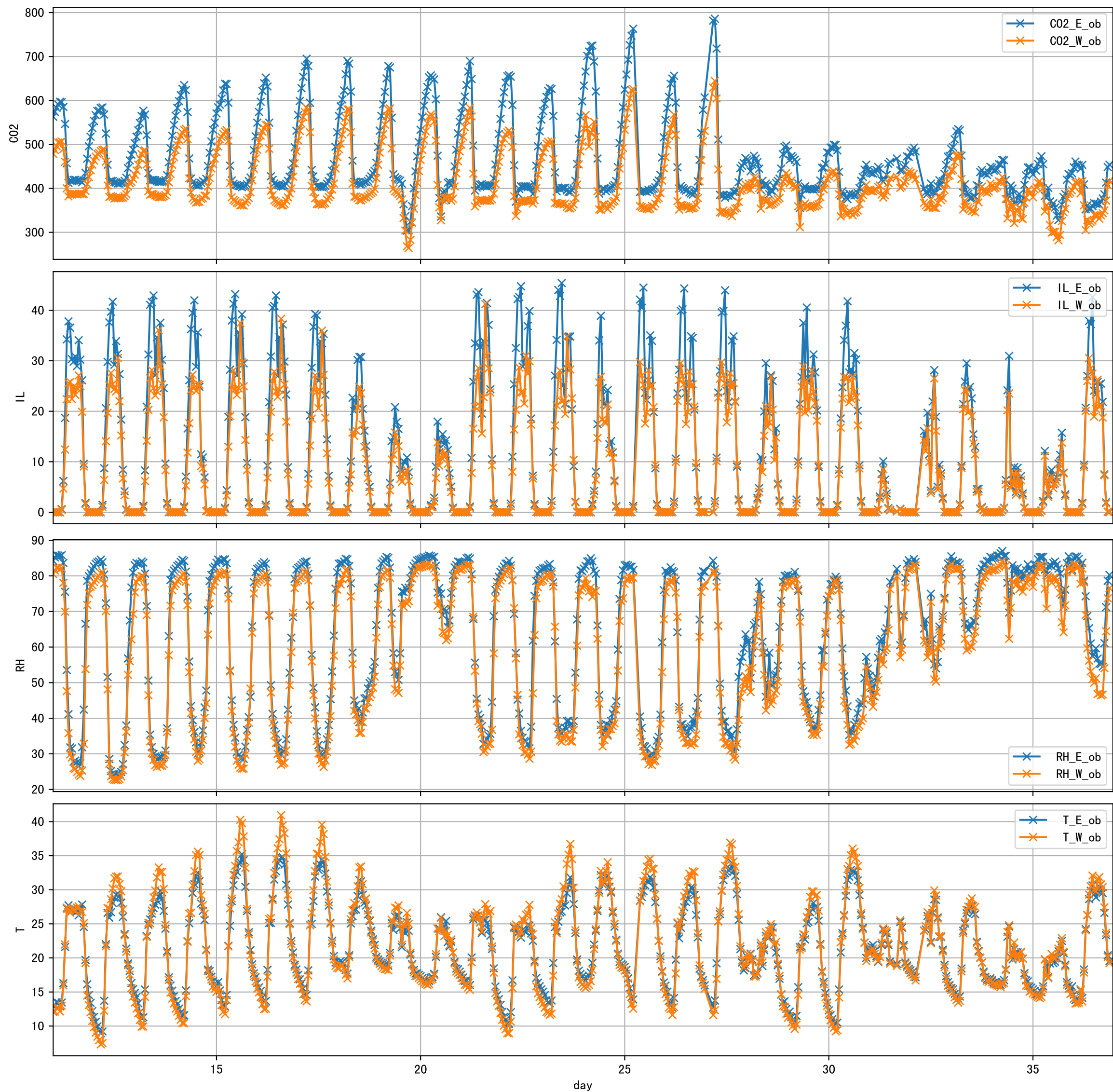
G3-4 2025-05-12 IA Observed Sensor Data
