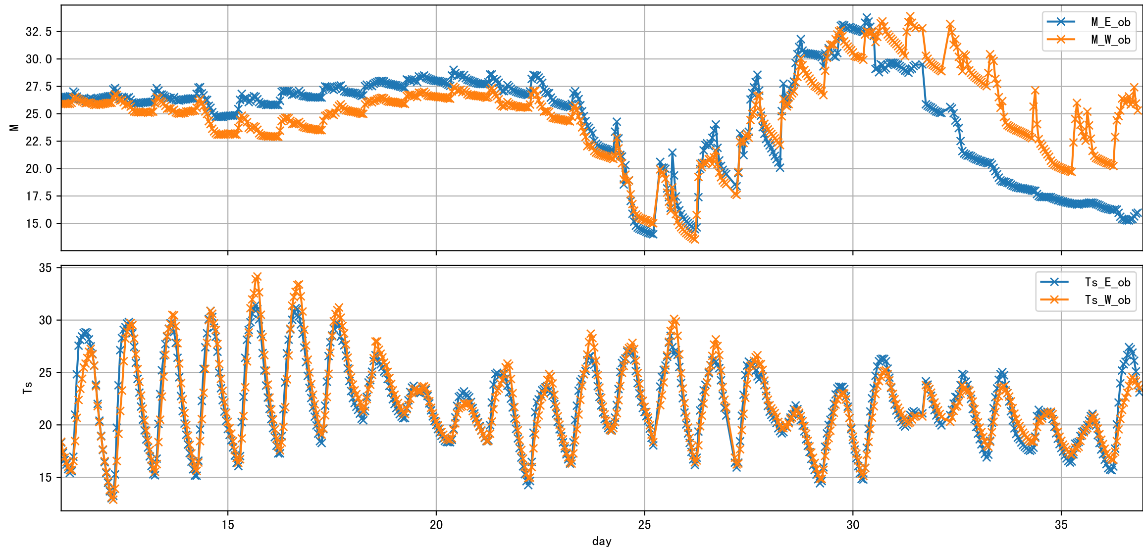
G3-4 2025-05-12 IS Observed Sensor Data
