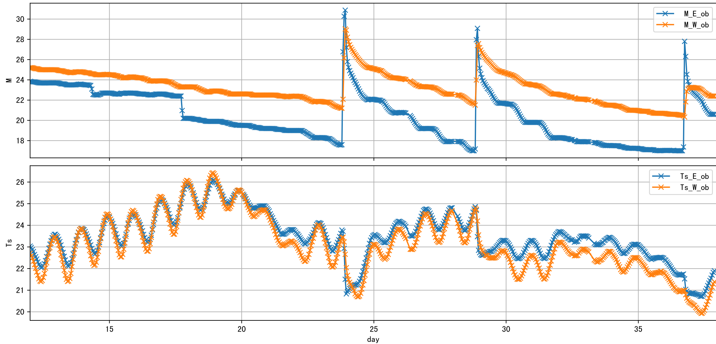
G3-5 2025-05-11 IS Observed Sensor Data
