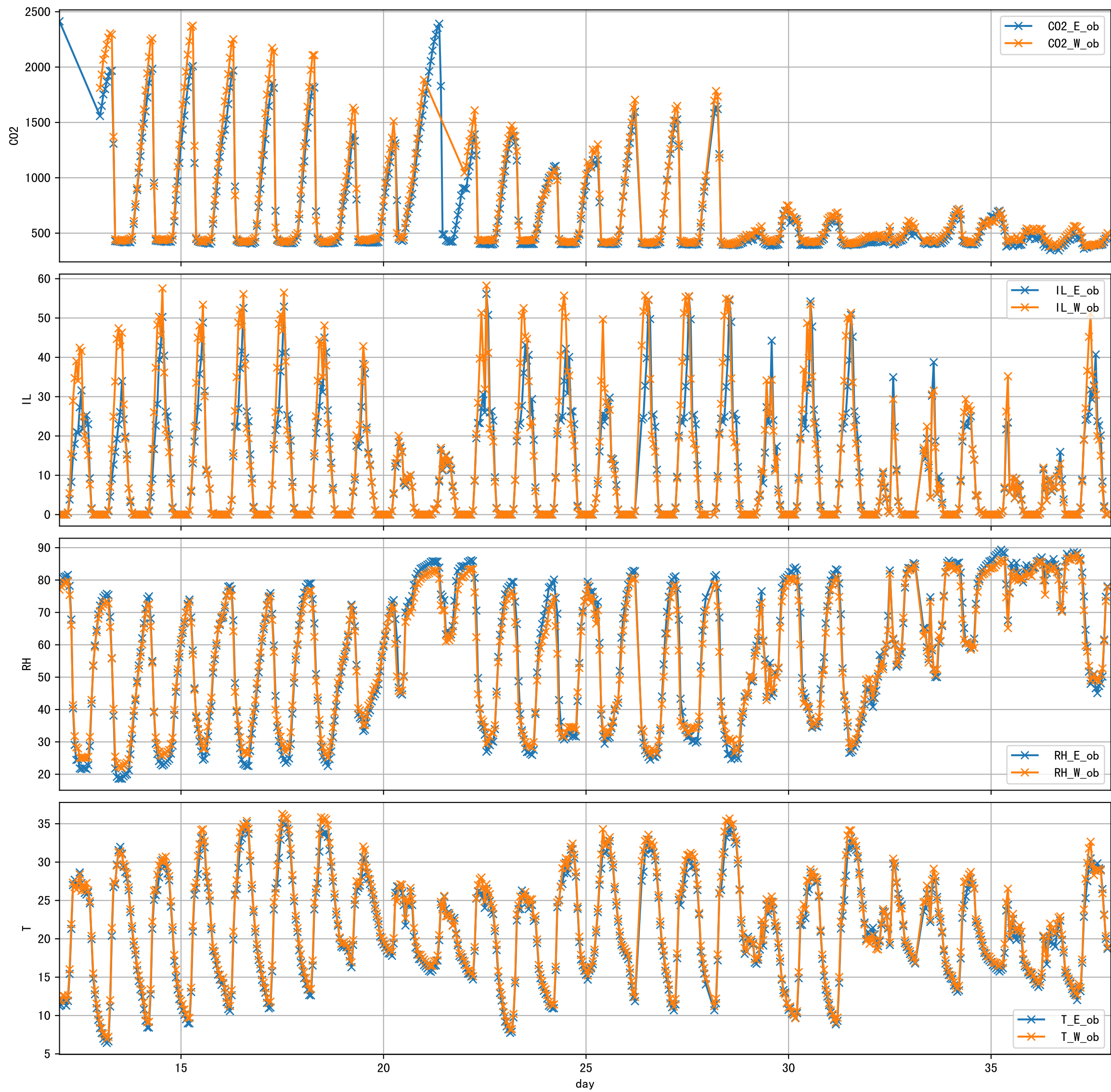
G3-5 2025-05-11 IA Observed Sensor Data
