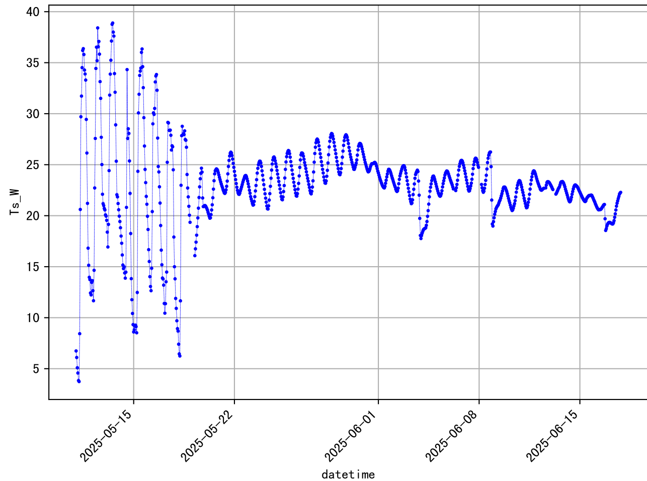
'H' data (37 days, 61 min/dp) 102363@102314IS_Ts_W
