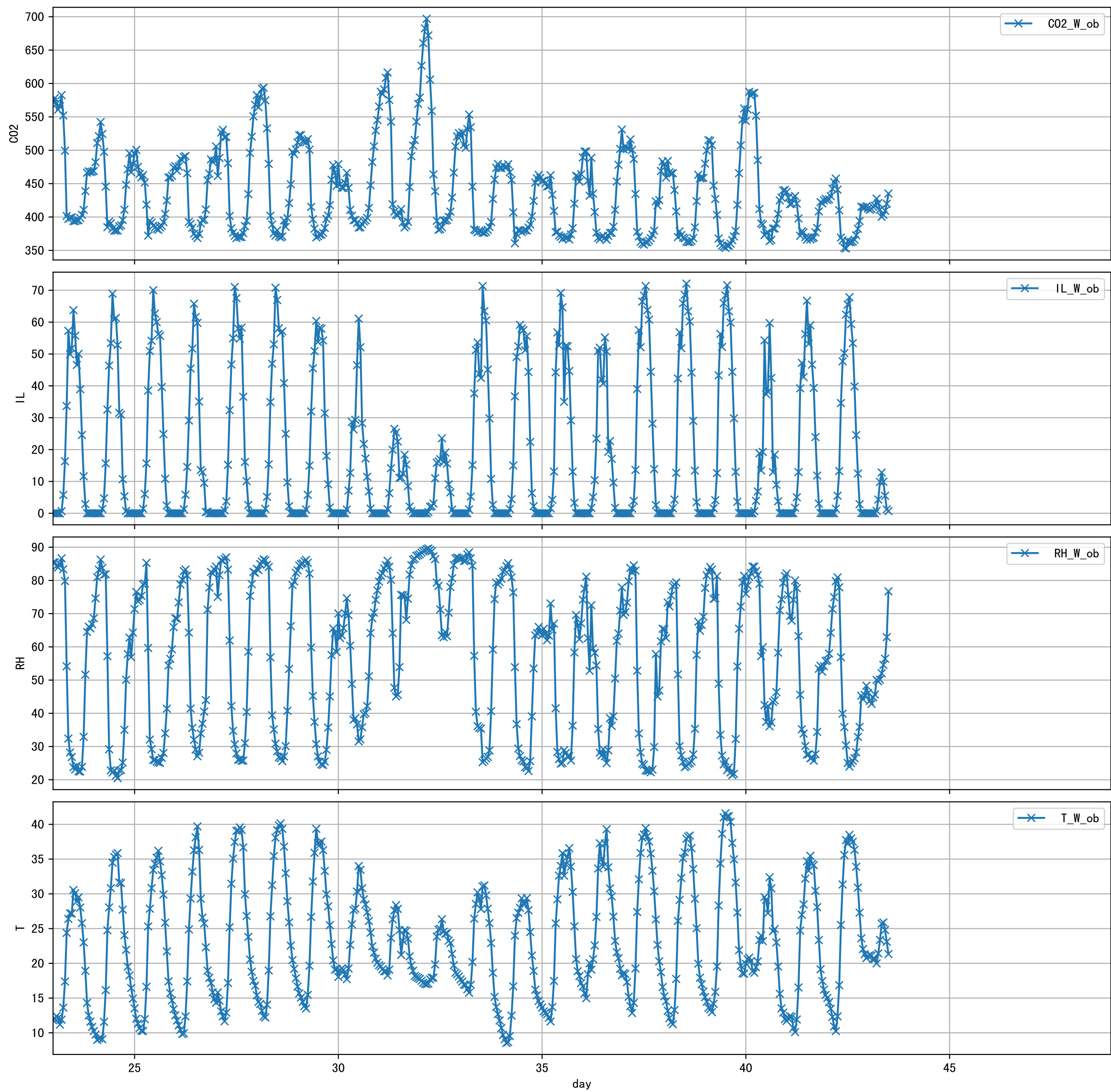
MG 2025-04-30 IA Observed Sensor Data
