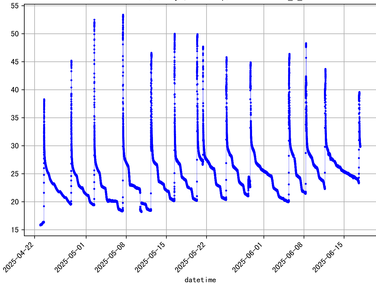
'Raw' data (55 days, 1 min/dp) 8752@8997IS_M_E
