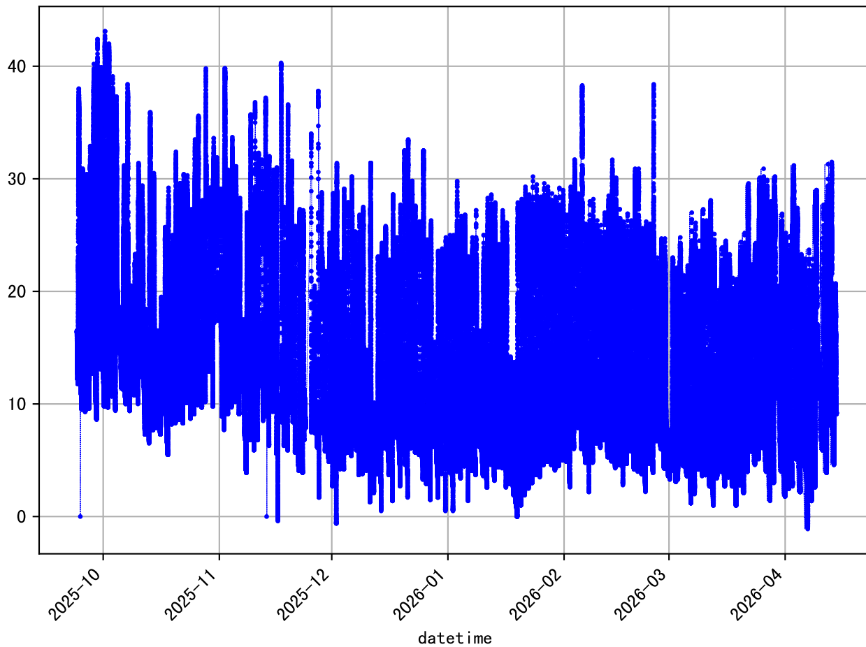
'Raw' data (201 days, 1 min/dp) 106849@3501A_T_E
