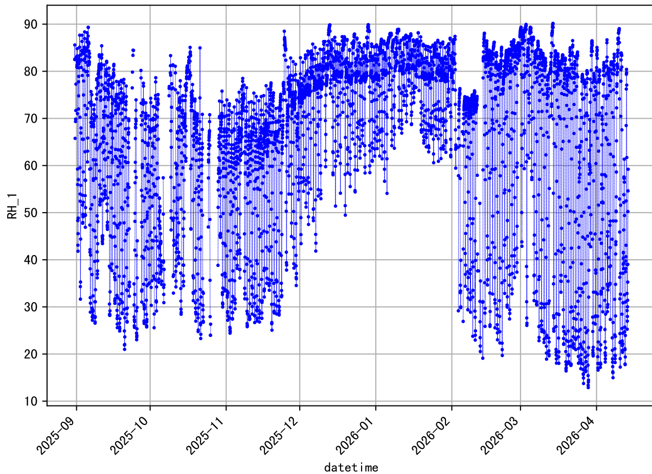
'H' data (225 days, 64 min/dp) 934@11711A_RH_1
