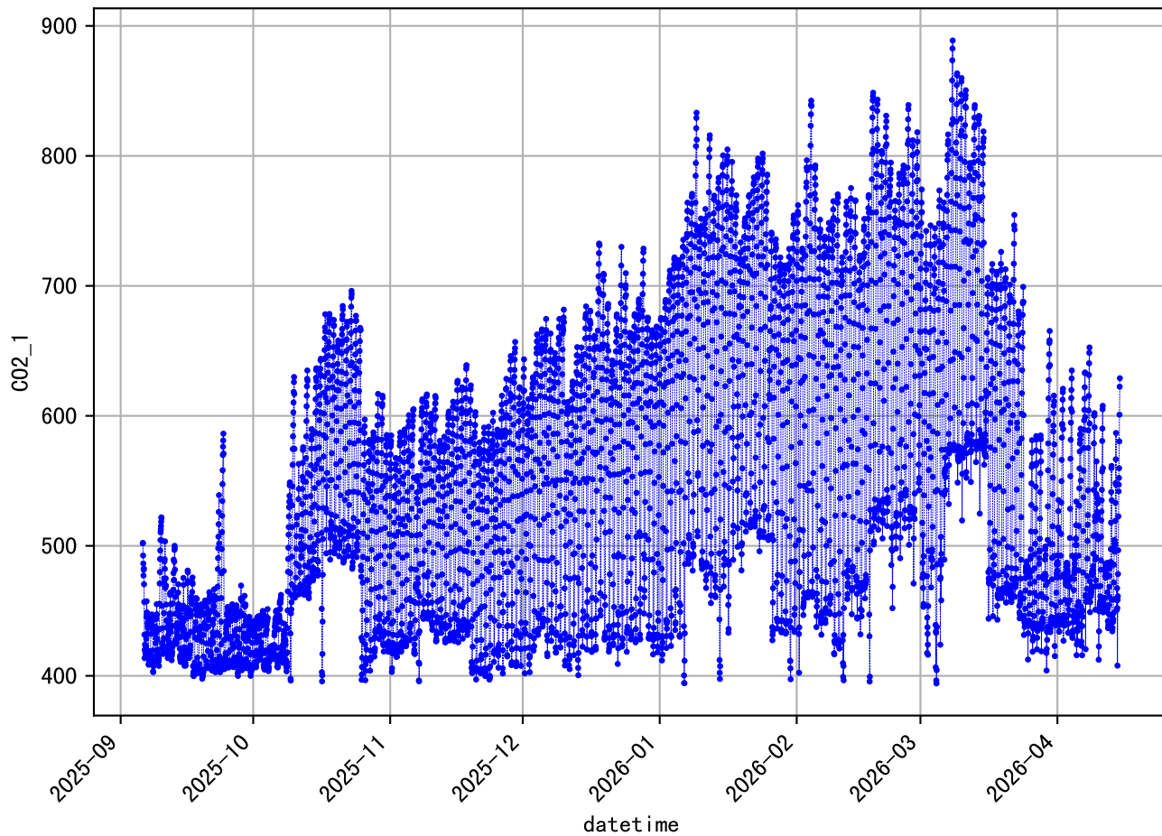
'H' data (221 days, 60 min/dp) 959@11961A_C02_1
