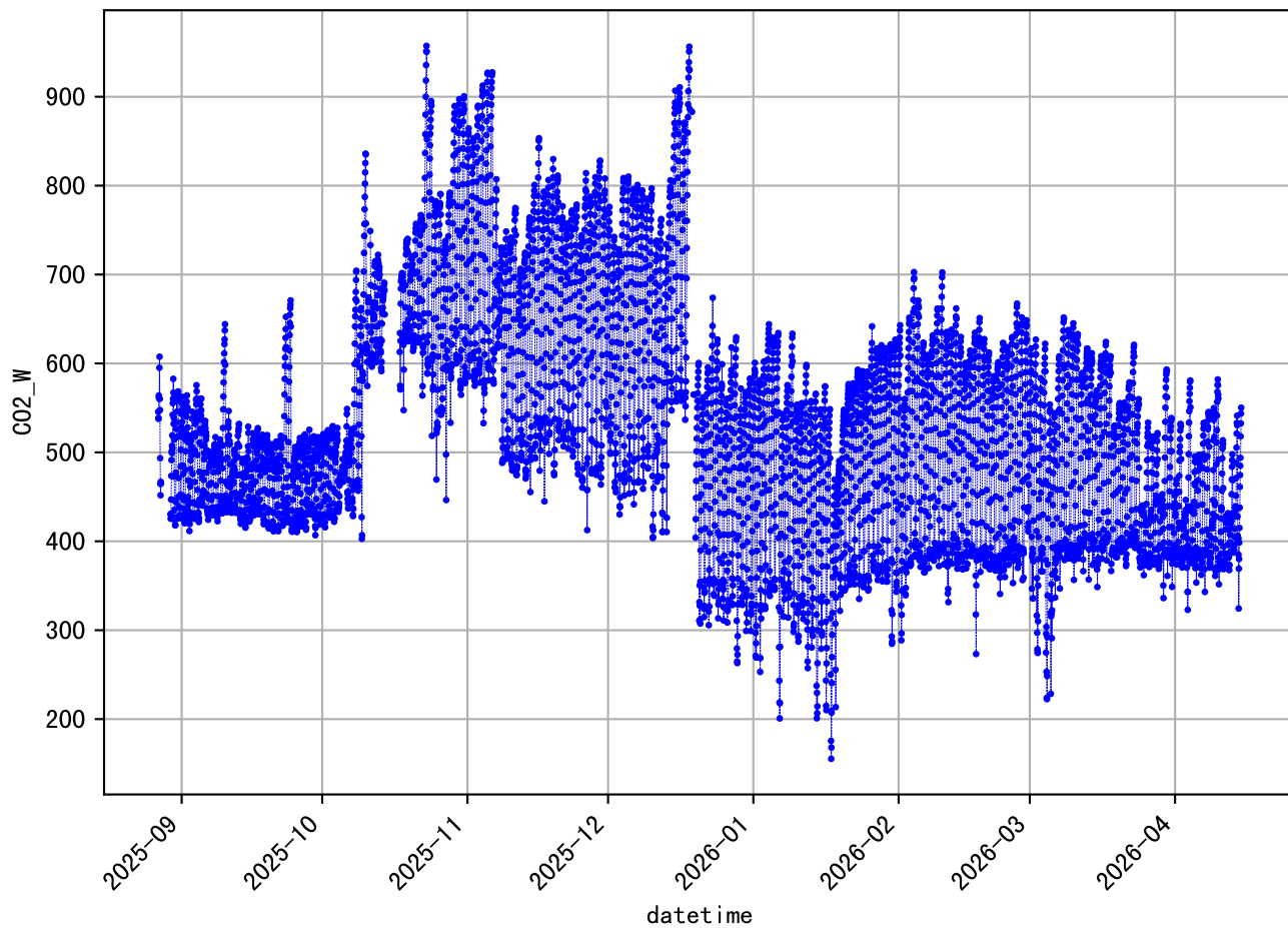
'H' data (231 days, 61 min/dp) 851@1088IA_C02_W
