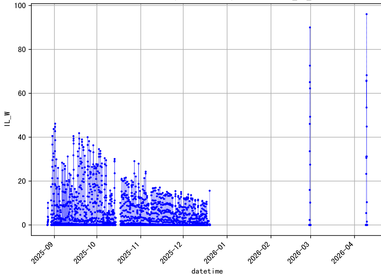
'H' data (225 days, 122 min/dp) 852@1089IA_IL_W
