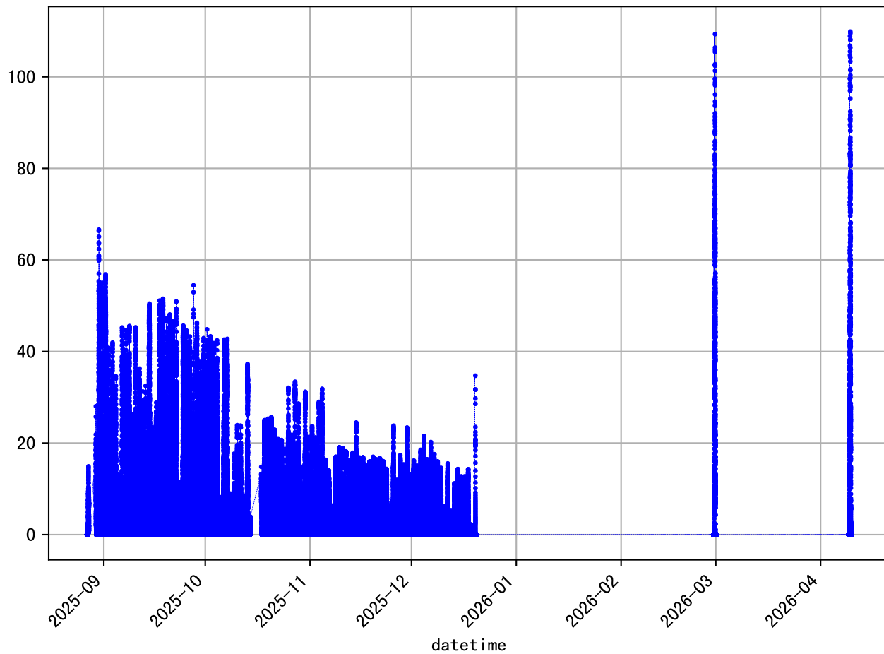
'Raw' data (225 days, 2 min/dp) 852@1089IA_IL_W
