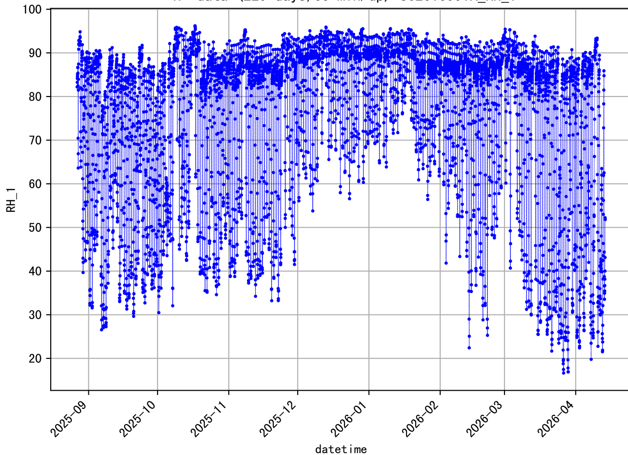
'H' data (229 days, 60 min/dp) 862@10991A_RH_1
