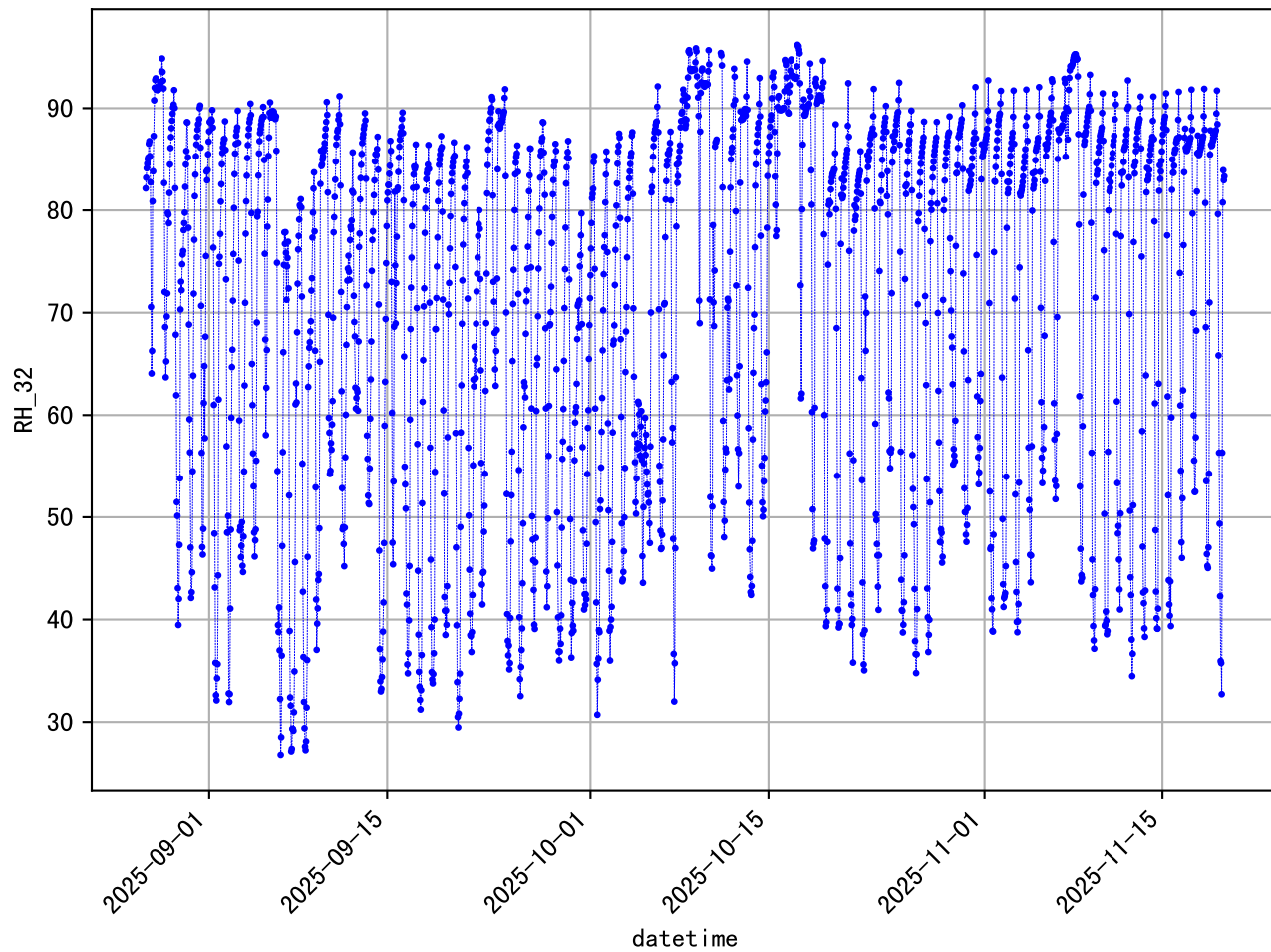
'H' data (84 days, 60 min/dp) 862@10991A_RH_32
