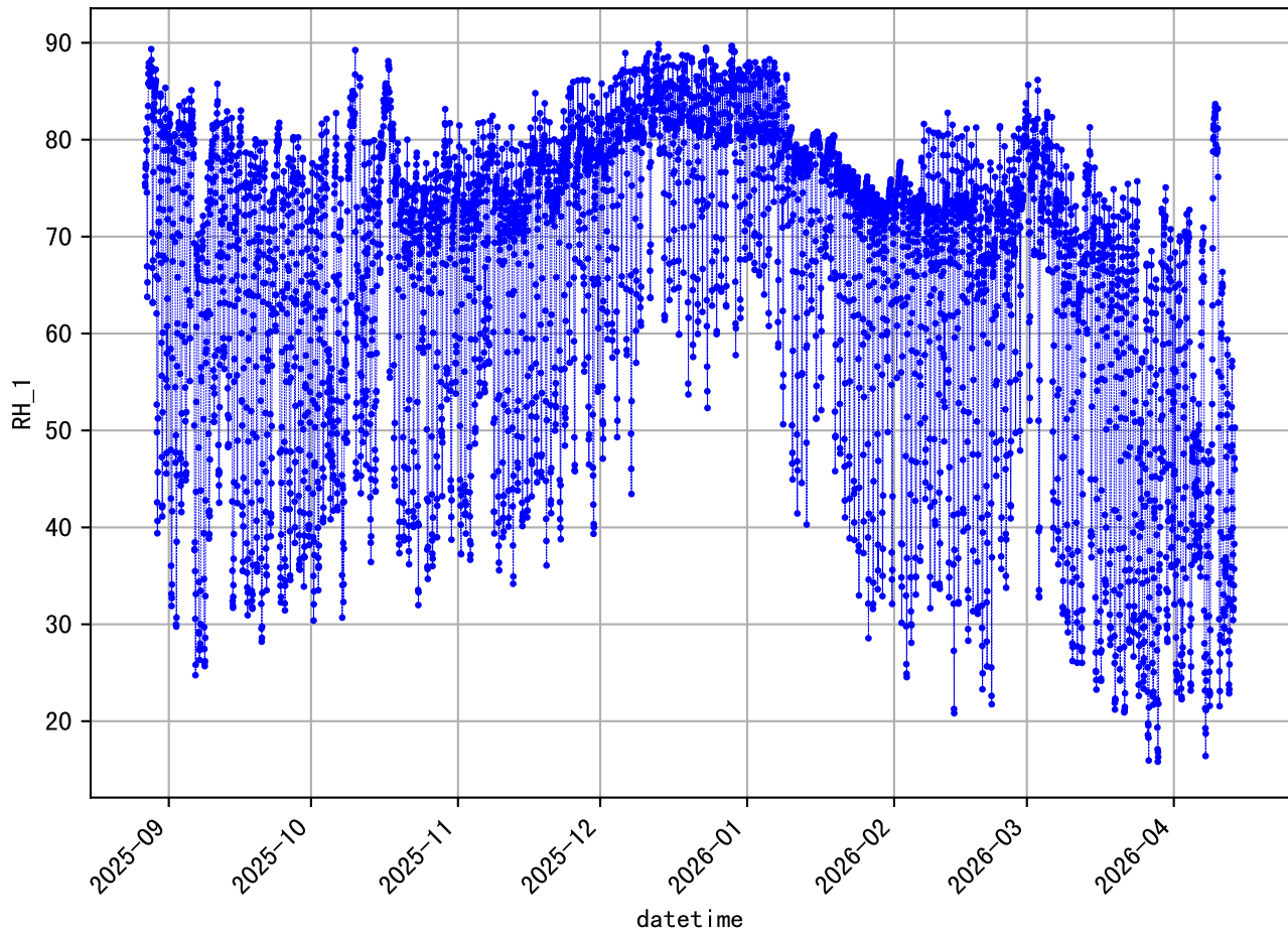
'H' data (229 days, 60 min/dp) 874@11111A_RH_1
