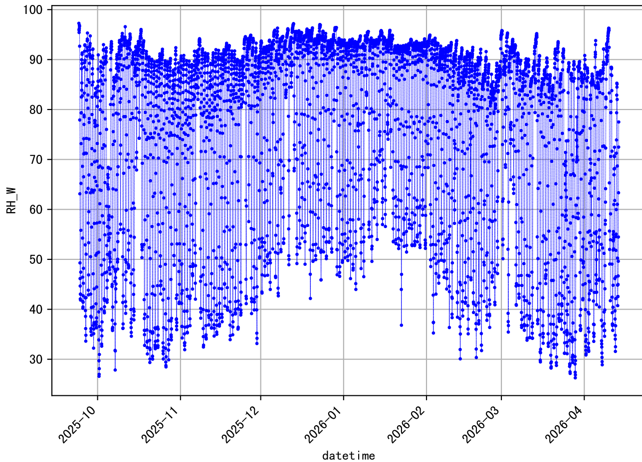
'H' data (201 days, 60 min/dp) 8648@88931A_RH_W
