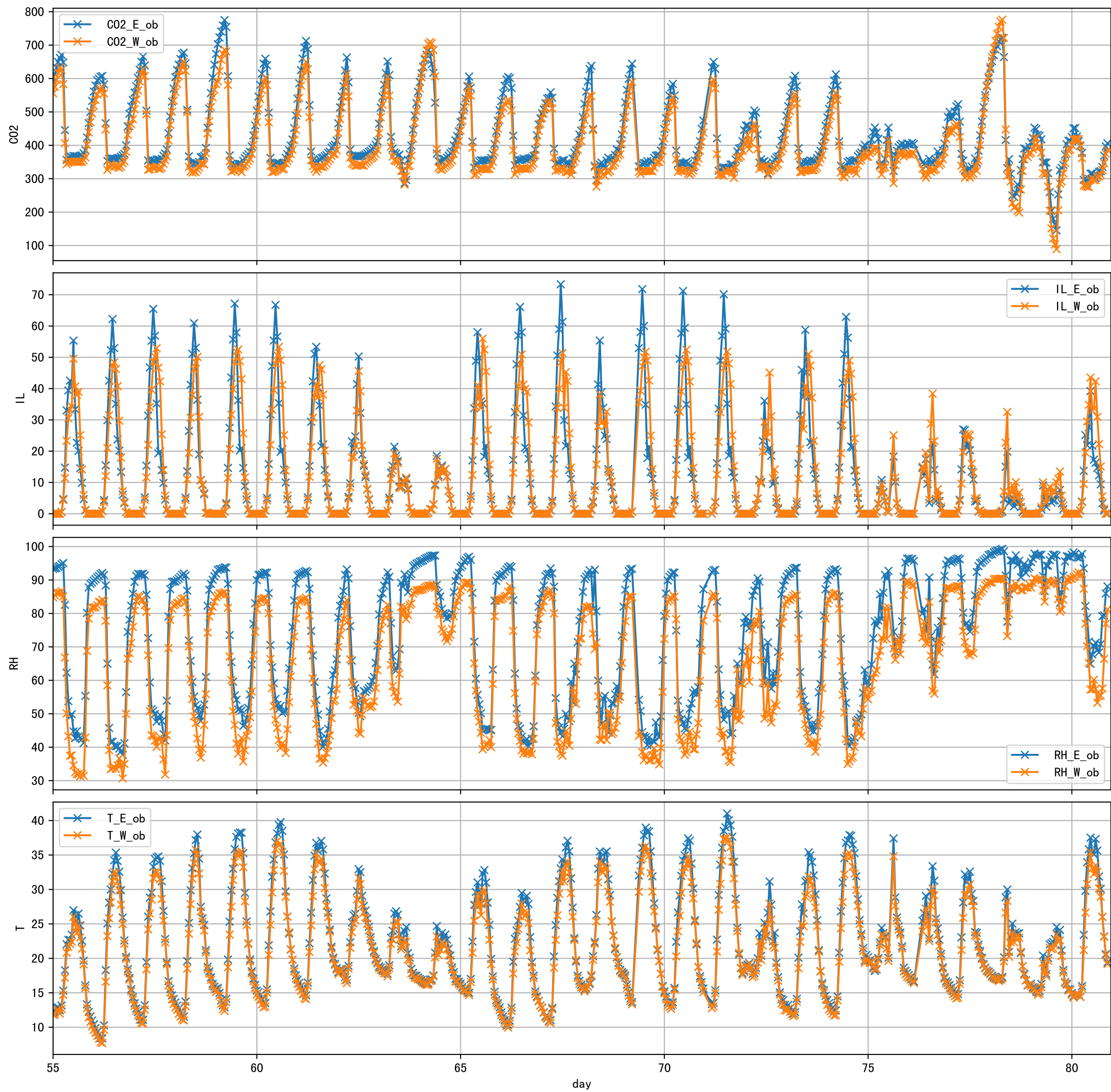
P3-8 2025-03-29 IA Observed Sensor Data
