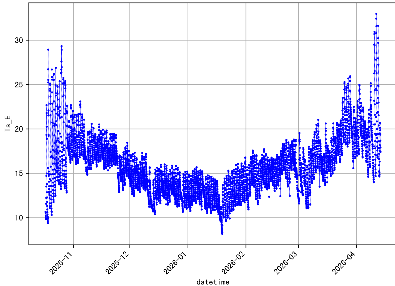
'H' data (178 days, 60 min/dp) 8703@8948IS_Ts_E
