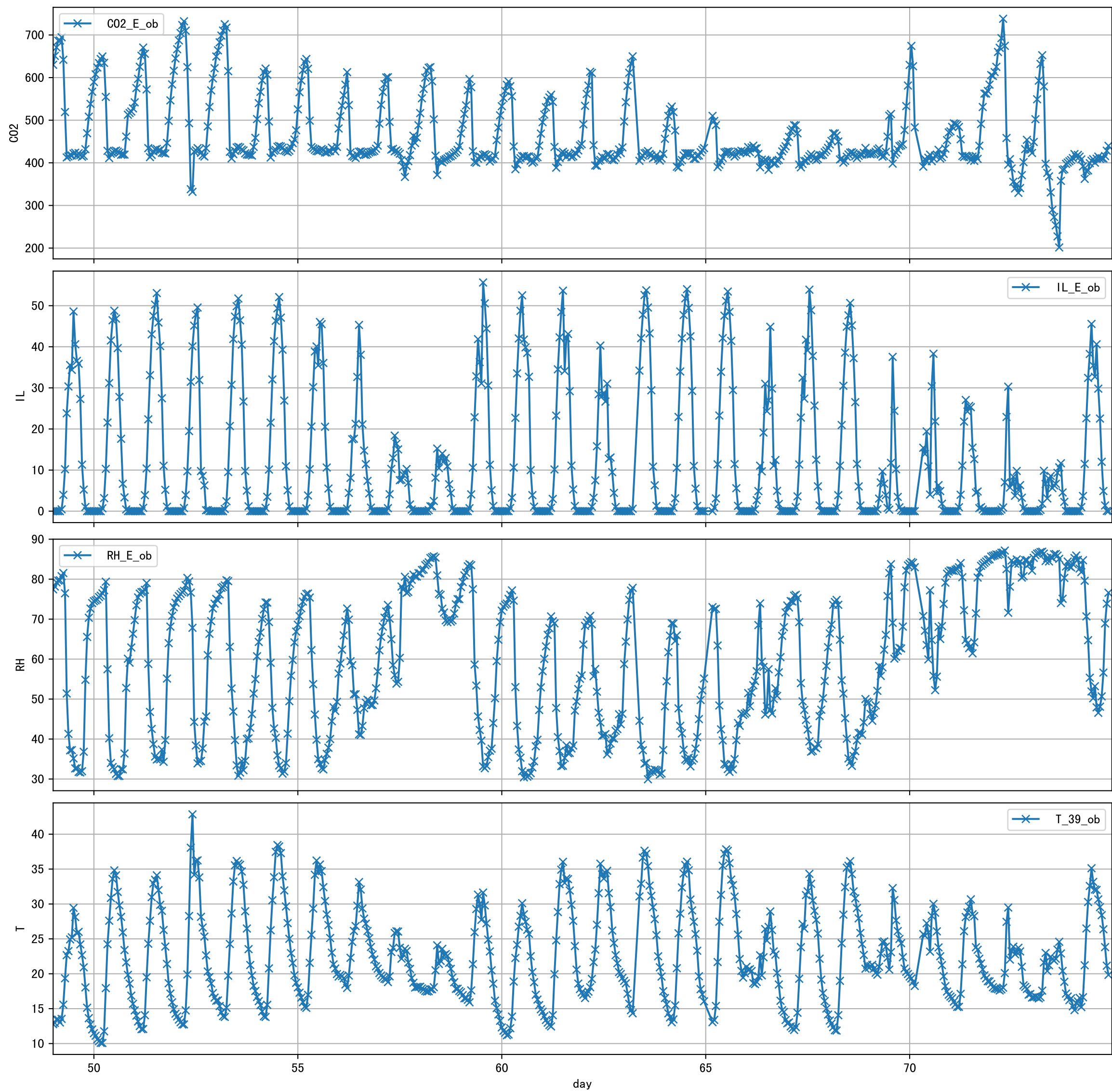
P8 2025-04-04 IA Observed Sensor Data
