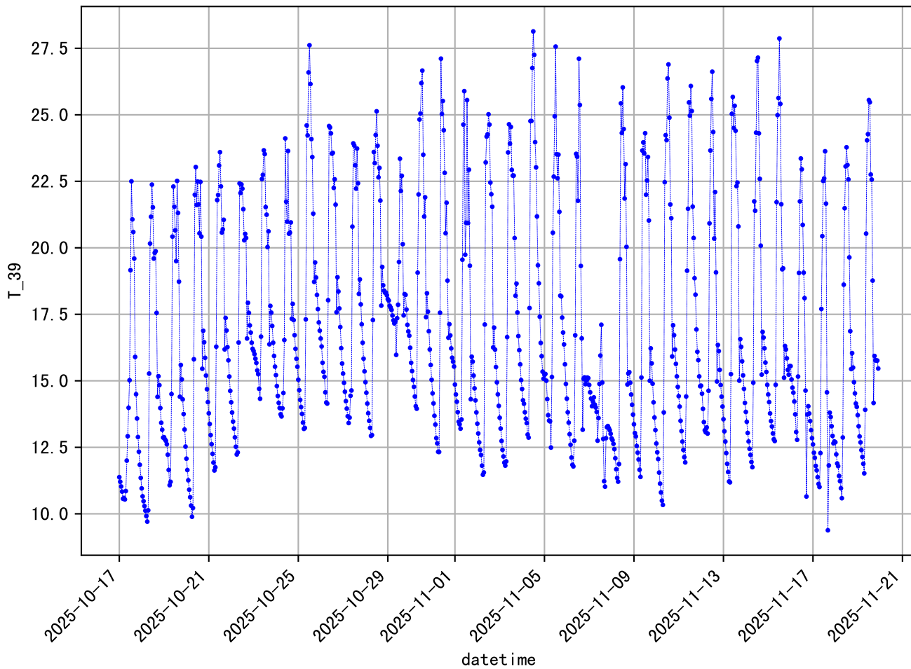
'H' data (33 days, 59 min/dp) 100105@3761A_T_39
