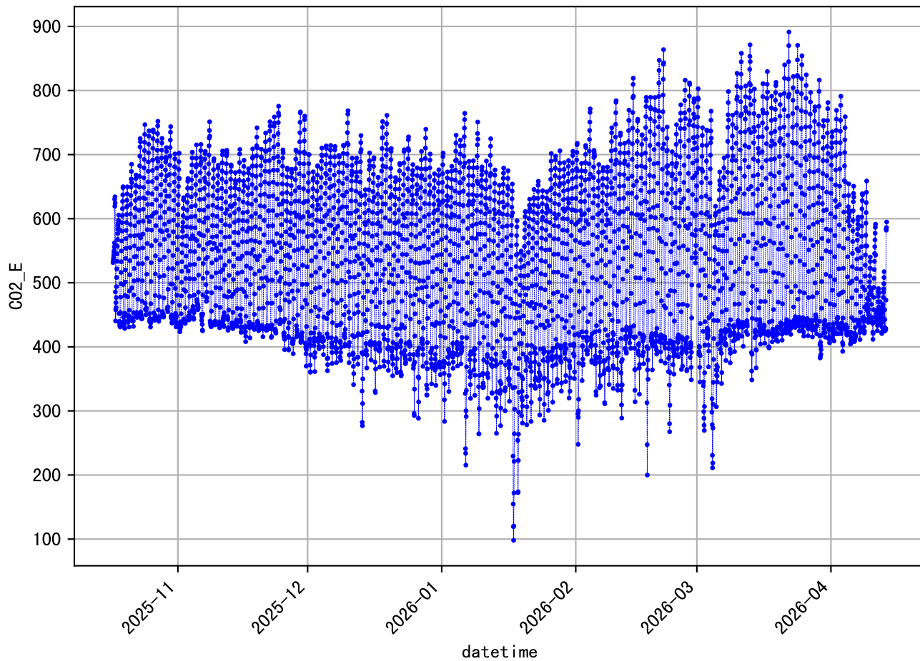
'H' data (178 days, 59 min/dp) 8711@89561A_CO2_E
