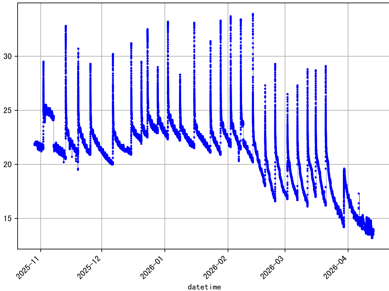
'Raw' data (166 days, 1 min/dp) 8716@8961IS_M_E
