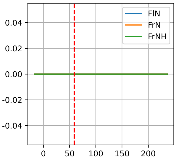
L1A4: ['FIN', 'FrN', 'FrNH']
