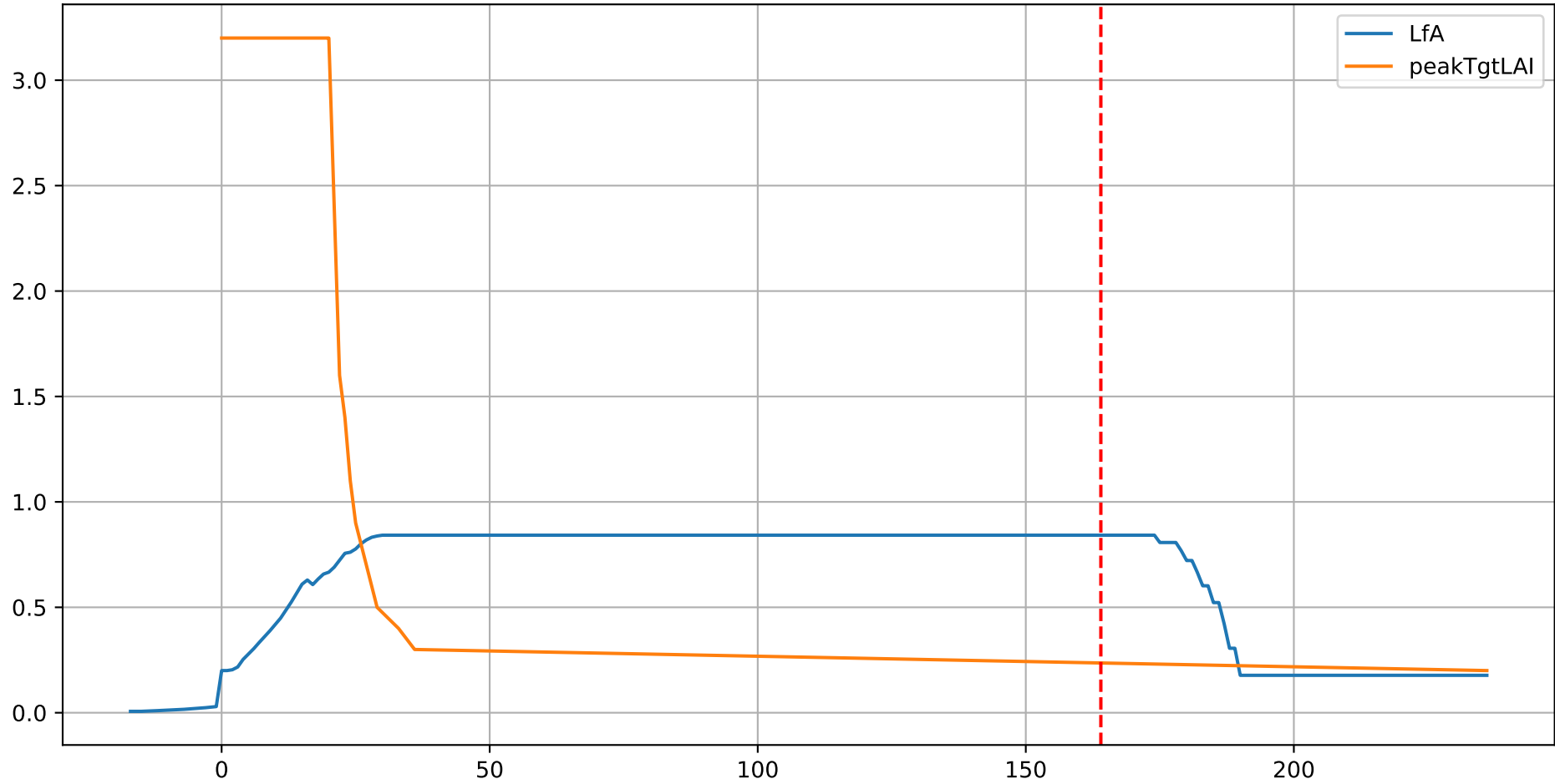
L1AC1: ['LfA', 'peakTgtLAI']
